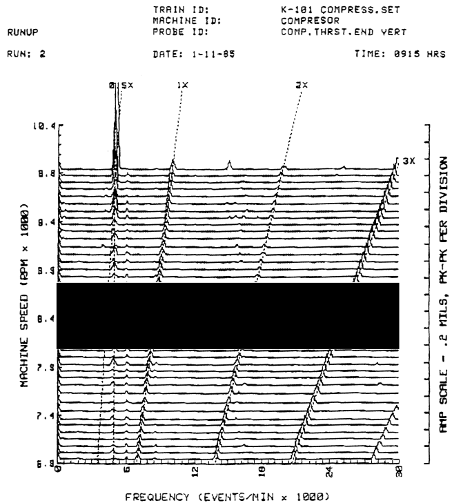
Figure 16. Subsynchronous Vibrations with Dry Gas Seals [11].
