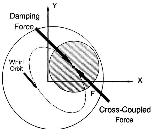
Figure 3. Crosscoupled Stiffness and Damping Force.
