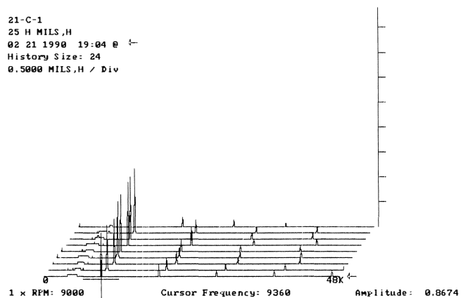
Figure 26. Vibration Spectrum with Honeycomb Seals.
