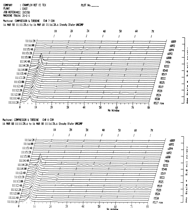
Figure 23. Cascade Spectrum Showing High Subsynchronous Vibration.
