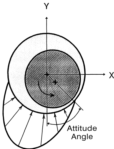
Figure 1. Hydrodynamic Pressure Profile in a Journal Bearing.
