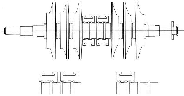
Figure 7. Balance Piston Labyrinth Initial Modification.
