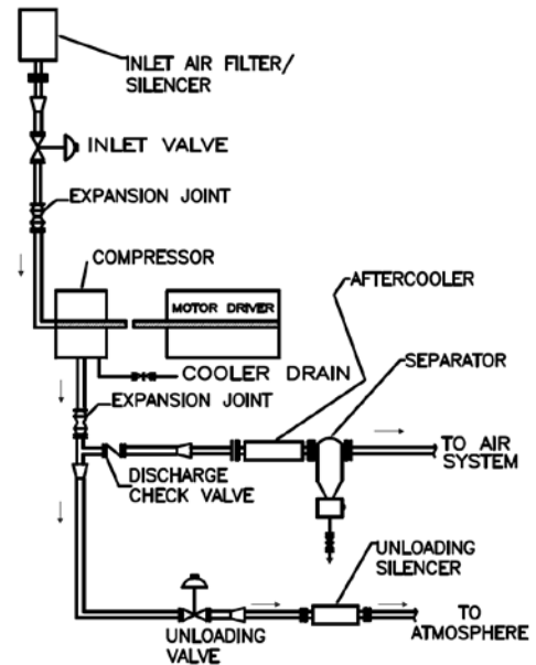
Figure 4. General Arrangement of Accessories and Hardware.
