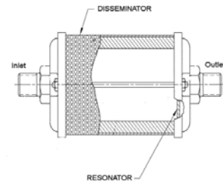
Figure 14. Drain Muffler.
