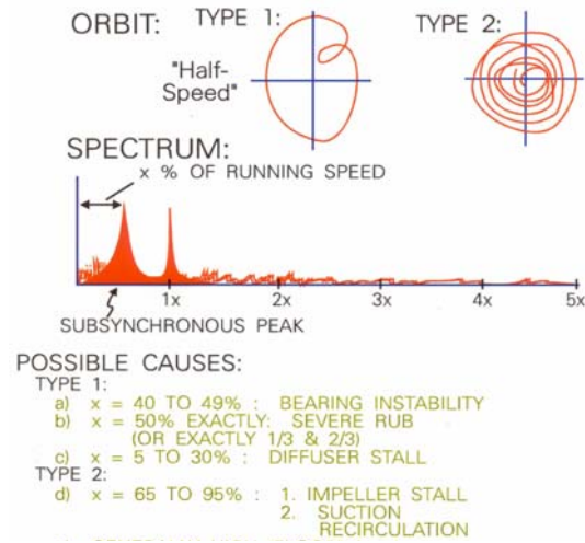
Figure 9. Subsynchronous Vibration
