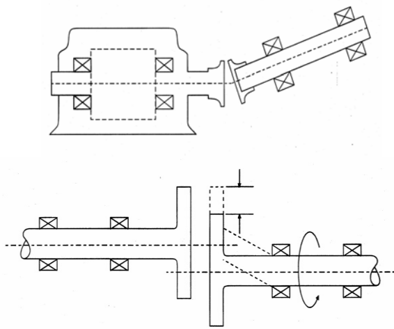
Figure 6. Illustration of Angular and Offset Misalignment
