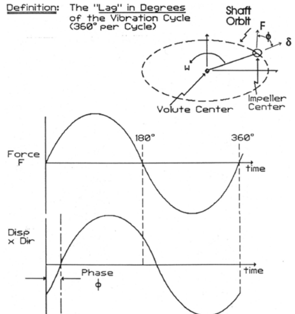
Figure 2. Definition of Phase Angle
