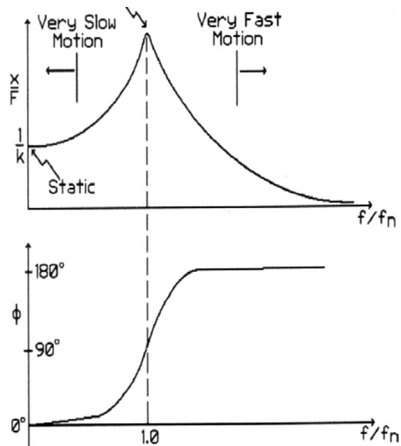
Figure 3. Relationship of Phase Angle to Frequency
