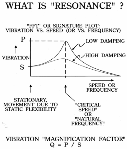
Figure 1. Illustration of Natural Frequency Resonance, and Effects of Damping
