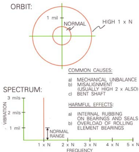
Figure 5. Imbalance Example of Shaft Orbit and FFT Spectrum Pump/ Driver Alignment
