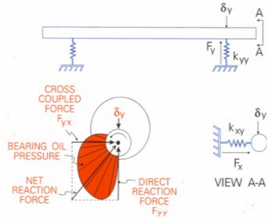
Figure 10. Cross-Coupled Stiffness Subsynchronous Whirl & Whip
