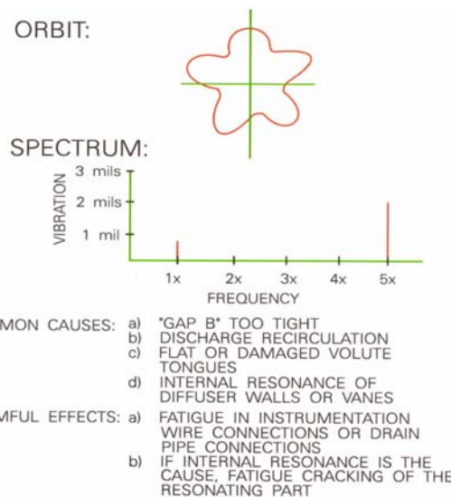
Figure 12. Vane Pass Vibration
