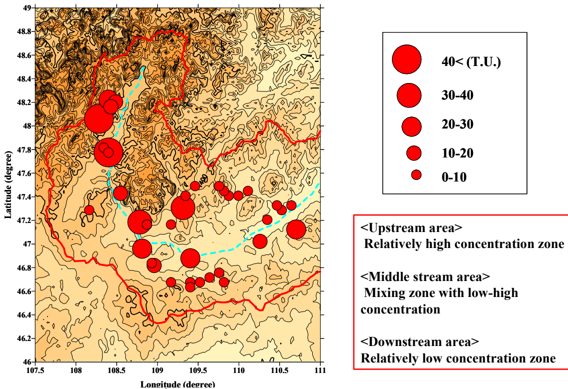
Fig. 2 Spatial distribution of ^3\text{H} concentration in the groundwater of Kherlen River basin in 2002 and 2003 (Higuchi et al., 2004).
