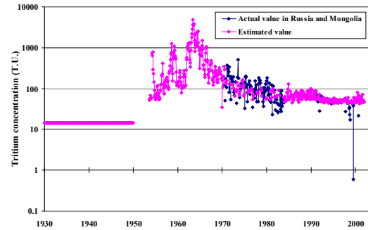
Fig. 1 Temporal change of ^3\text{H} concentration of precipitation in Mongolia (Higuchi et al., 2004).
