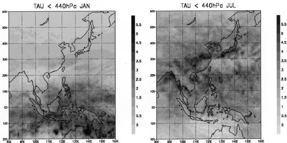
Fig.3. Cloud optical thickness for high cloud ( cloud top < 440 hPa ) in 1996.
