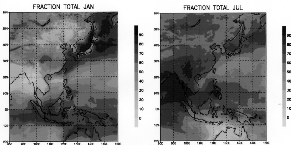
Fig.1. Monthly averaged cloud fraction from GMS-5.
