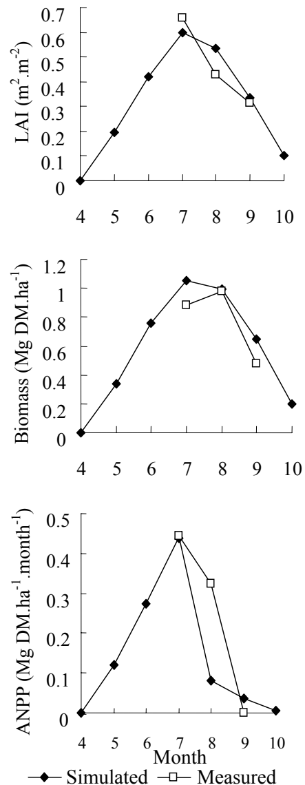
Fig. 2 Simulated and measured data at KBU.
