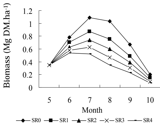
Fig. 3 Effect of grazing on aboveground biomass.
