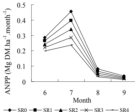
Fig. 4 Effect of grazing on aboveground net primary production.
