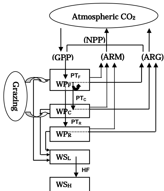
Fig. 1 Model structure of Sim-CYCLE (Ito and Oikawa, 2000).
