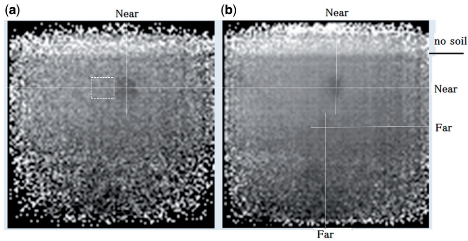
Fig. 3. Images of muon yield distributions obtained (a) with a 2 m cubic near iron block only over 5 days, and (b) with a 1 \times 2 \times 2 m 3 near block and a 2 m cubic far block over 67 days. The absorption due to the object is indicated by the shadow and the locations of the blocks are indicated by the lines. In (a), the location of “air” is indicated by the dash-lined box. This is subtracted from the absorption observed in the iron block region to obtain the absorption due to only the iron block.
