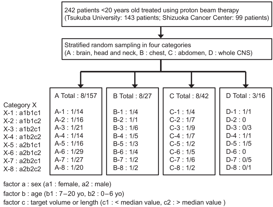
Figure 1. Schema of stratified random sampling from patients who had been treated using proton beam therapy at the Tsukuba University Hospital or Shizuoka Cancer Center.
