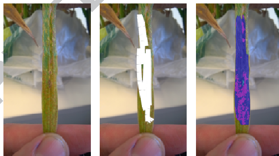
Figure 8: Leaf mask refinement algorithm (left) original image, (center) input mask given by a user through the smartphone app (right) in blue, the refined mask (blue) with the detected diseases (other colors)
