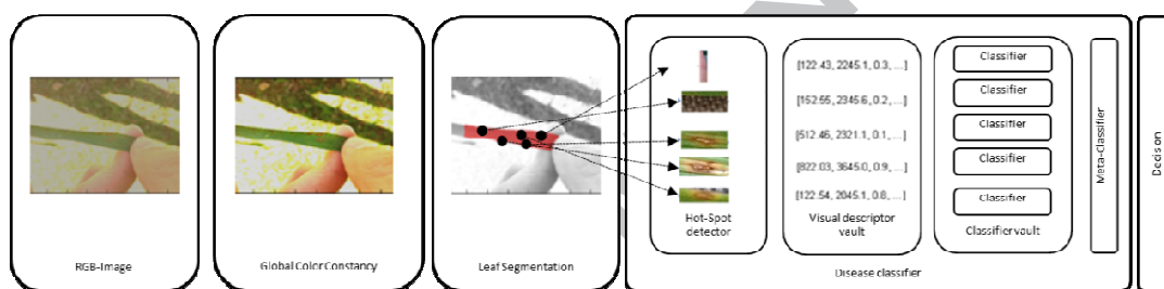
Figure 5: Global algorithm layout
