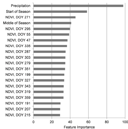
Figure 8. Mean feature importance of the 20 most important features for the years 2001–2014 scaled between 0 and 100.
