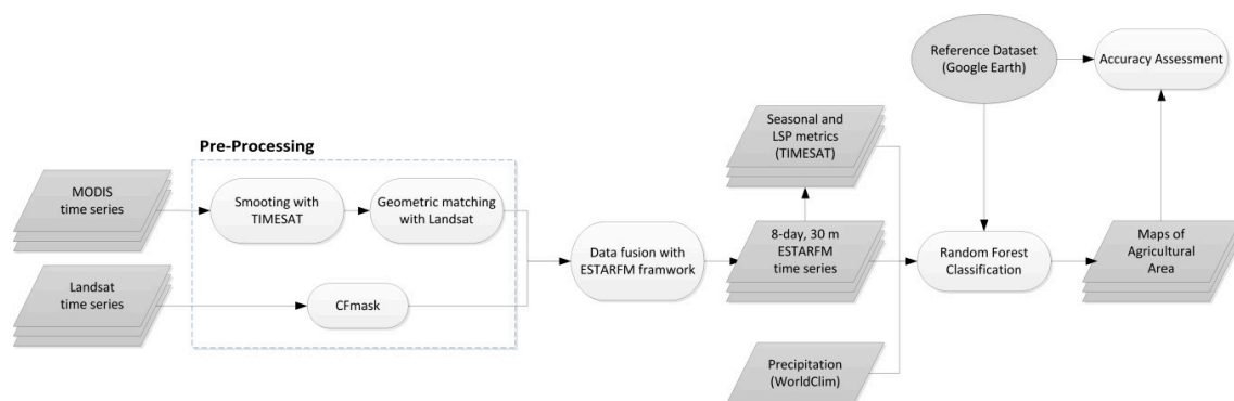
Figure 3. Workflow of pre-processing, data fusion, and classification for the generation of maps of agricultural area for entire Burkina Faso.
