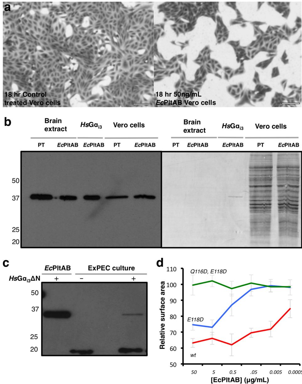
Figure 2. Cytotoxicity of recombinant EcPitAB. 18 h after treatment with buffer or different concentrations of EcPitAB, Vero cells were stained and imaged. a , representative images for untreated controls ( left ) and 50 ng/ml EcPitAB ( right ) are shown. b , ADP-ribosyltransferase assays in which pertussis toxin or EcPitAB were used to modify different protein substrates, including trimeric G-protein extracts, recombinant human G \alpha_{13} , or Vero cell lysates. Reactions at 37 °C were performed in the presence of biotin-NAD + and then quenched after 5 min, separated by SDS-PAGE, transferred to a Western blotting membrane, and imaged with either luminescence following streptactin-HRP exposure ( left ) or Coomassie ( right ). c , Western blottings showing the incubation of ExPEC culture medium with NAD + -biotin with and without the presence of HsG \alpha_{13} ΔN. d , Vero cells were imaged in a similar manner to those in a were monitored for the degree of cell growth relative to buffer controls following exposure to different concentrations of EcPitAB or A subunit mutants. Surface area is calculated from the percentage of each image stained by crystal violet. Data represent the mean \pm S.D. from three replicates.
