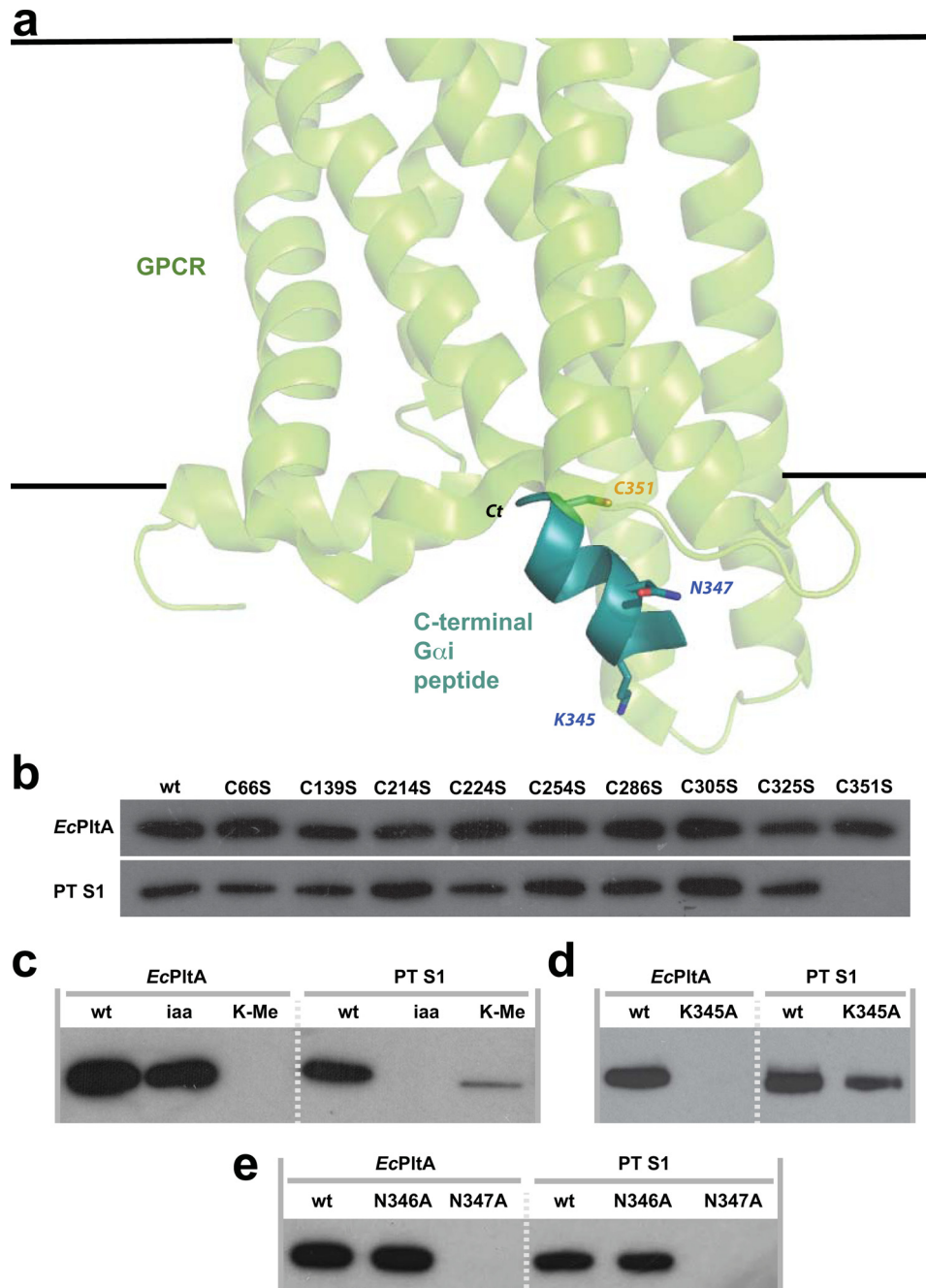
Figure 4. Proposed model of the pertussis-like toxins transfer target. a , structure of opsin in complex with the C terminus of transducin (Scheerer et al. (38), Protein Data Bank code 3DQD); their K345L mutant was reverted to lysine for this figure. G\alpha_i is shown in teal; the position of the C terminus and ADP-ribosylated residues discussed in text are shown. The plasma membrane and GPCR (green) are at the top. b , ADP-ribosyltransferase assays using EcPltA or pertussis toxin in which potential acceptor cysteines within G\alpha_i\Delta N were mutated to serine; or c , following iodoacetamide and lysine methylation; d , mutation of Lys-345; or e , Asn-346 and Asn-347 to alanine.
