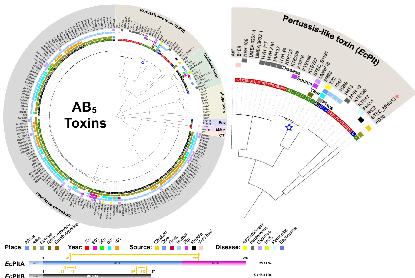
Figure 1. E. coli AB 5 toxins. Shown is a cladogram of AB 5 toxin sequences identified in genome sequenced E. coli strains available on the NCBI database. Archetype sequences from the querying dataset are indicated with an asterisk. E. coli strains harboring more than one AB 5 group are indicated by a red star. The inner circle represents the E. coli phylogenetic groups (A, B1, B2, and D). Additional color-coded circles indicate the place, year, and source of each strain, as well as the associated infection (where known). Because Shiga toxigenic E. coli strains are over-represented in the NCBI database, only archetypical Shiga toxin variants are presented. The EcPitA toxin focused on in this study is highlighted with a blue star. A schematic of the A and B subunit domain displayed with the positions of the intramolecular disulfides (yellow) and the inhibitory C terminus (pink) is at the bottom of the figure. Inset, an expanded view of the pertussis toxin branch. A complete overview of all Shiga toxin variants and their associated strains is presented in supplemental Fig. S1.
