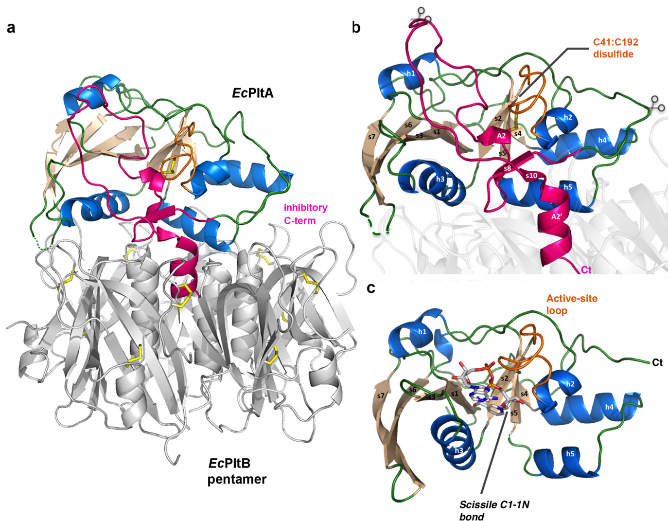
Figure 6. Activation mechanisms of EcPltA and cholera toxin. a , schematic representation of the EcPltA B holotoxin in which \alpha -helices are colored marine , \beta -strands wheat , and loop regions green . The C-terminal A2 domain is highlighted in pink showing its interaction with the B subunits of the glycan-binding pentamer ( gray ). b , schematic representation highlighting the holotoxin's EcPltA subunit. The conserved redox-sensing disulfide is labeled, and the rough position of the B-pentamer is shown as a partially transparent structure. Predicted potential proteolytic sites are shown with partially transparent scissors, and the C terminus is marked Ct. c , reduced active \text{NAD}^+ co-complex with all secondary structural elements labeled. The enzymatically cleaved N -glycosidic bond cleaved during the course of the reaction is highlighted.
