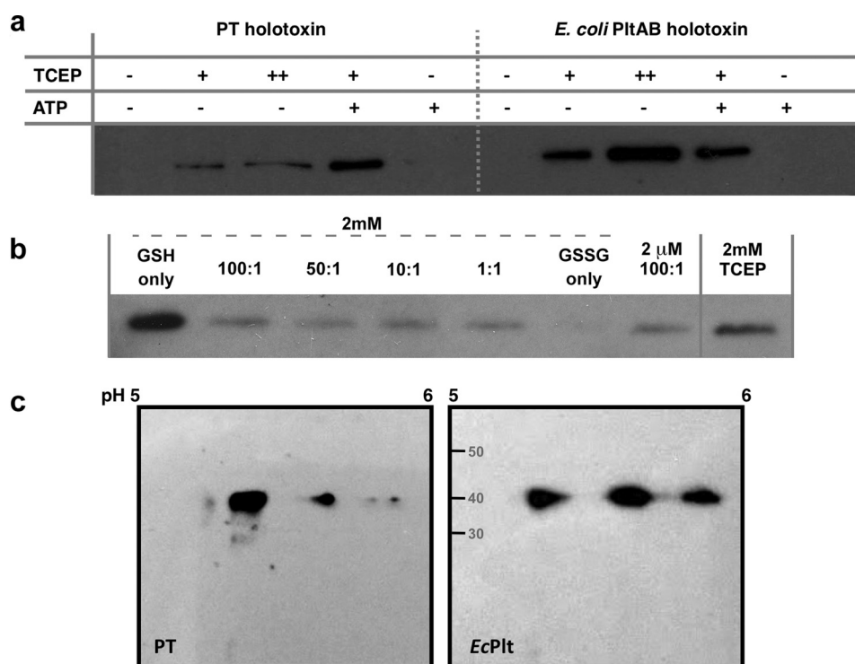
Figure 3. Activity assays for EcPltAB. a , ADP-ribosyltransferase assays similar to those used in Fig. 2 using biotinylated NAD + as a substrate to modify recombinant HsGα i3 ΔN PT ( left ) and EcPltAB ( right ) holotoxins were monitored for activity for 5 min at 37 °C in the presence of 10 mM (+) or 100 mM (++) TCEP and with or without 10 mM ATP. b , EcPltAB activation in the presence of different ratios of reduced (GSH) or oxidized (GSSG) glutathione within the ADP-ribosylation assay. c , 2D isoelectric focusing separation of different Ga i isoforms isolated from bovine brain extract following treatment with EcPltAB or PT indicate multiple Ga i isoforms act as substrates.
