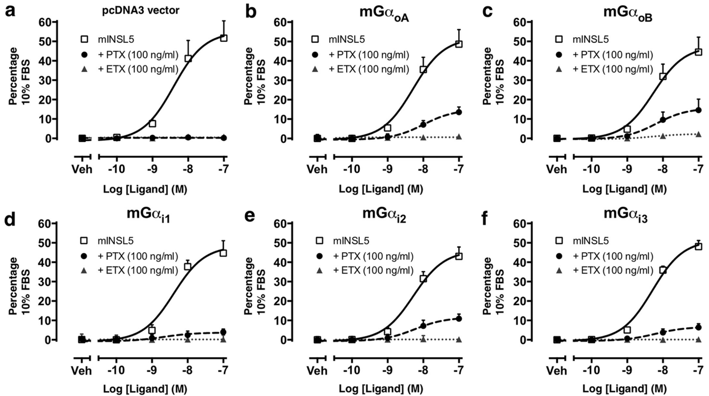
Figure 5. EcPltAB disrupts G-protein-coupled signaling. RFXFP4 recruits G_{i/o} \alpha subunits upon ligand activation. PT pretreatment abolishes INSL5-stimulated ERK1/2 phosphorylation, and this is rescued to differing degrees by transfection of individual PT-insensitive G_{i/o} mutants. a , Chinese hamster ovary-RFXFP4 cells were transiently transfected with pcDNA3 vector control, or b–f , G_{i/o} constructs carrying the C3511 mutation ( mG_{\alpha_{oA}} , mG_{\alpha_{oB}} , mG_{\alpha_{i1}} , mG_{\alpha_{i2}} , or mG_{\alpha_{i3}} ). Blockade of the response to PT but not EcPltAB pretreatment was rescued by transfection of the mutant G-proteins. Cells were stimulated with mouse INSL5 alone (0.1 to 100 nM) or after pretreatment with PT (100 ng/ml) or EcPltAB (100 ng/ml). Data points represent mean \pm S.E. of three independent experiments and are expressed as the % response of the positive control (10% v/v FBS). Veh , vehicle.
