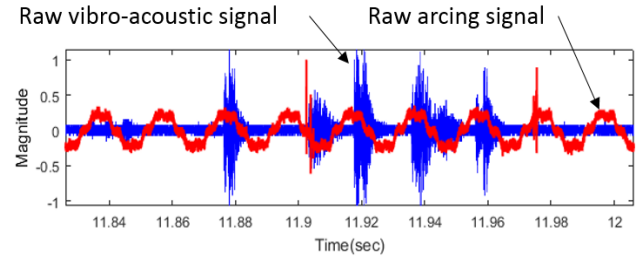
Fig. 2. Vibro-acoustic and arcing signals of an in-service OLTC at field.
