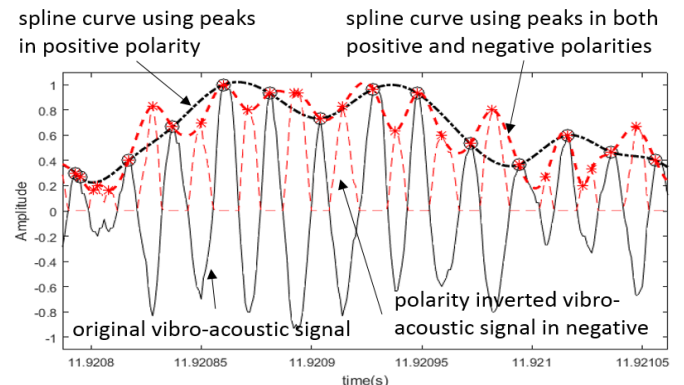
Fig. 4. (1) Spline curve using peaks in positive polarity (black dotted line); and (2) Spline curve using peaks in both positive and negative polarities (red dotted line).
