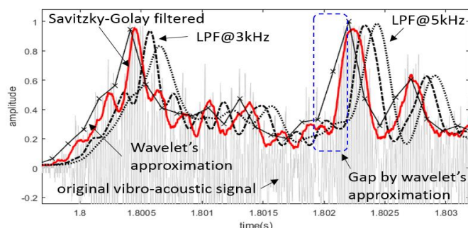
Fig. 11. Comparison of the time shifts in outputs of Savitzky-Golay filter, wavelet's approximation, and low-pass filter.
