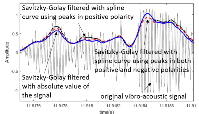
Fig. 5. Results of Savitzky-Golay filters with three different inputs as described in Fig. 4: (1) signal components with positive polarity (black dotted line); (2) signal components with both positive and negative polarities (red dotted line); and (3) absolute value of the vibro-acoustic signal (blue line).
