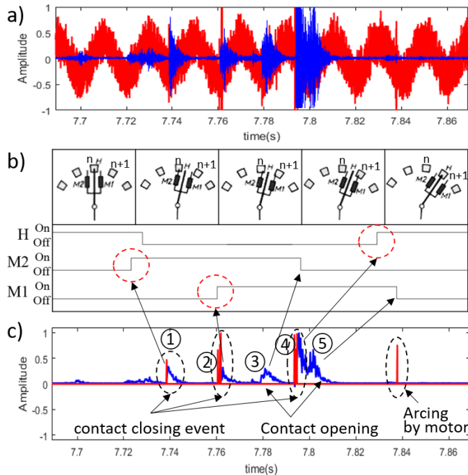
Fig. 18. (a) Originally measured vibro-acoustic signal (in blue) and arcing signal (in red) from a bolt-on type OLTC when it moves from the tap position n to the tap position n + 1 ; (b) timing diagram of the OLTC's contacts; and (c) results of Savitzky-Golay filtering on vibro-acoustic and arcing signals (red impulses are the arcing signals extracted and blue signals are the vibro-acoustic signals smoothed by Savitzky-Golay filters). H – main contact, M1 – transition contact, M2 – transition contact.
