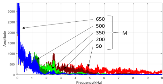
Fig. 10. Frequency spectrum of the outputs of Savitzky-Golay filters with different data frame sizes ( M = 50, 200, 350, 500, 650 ) but the same order of polynomial ( N = 5 ).
