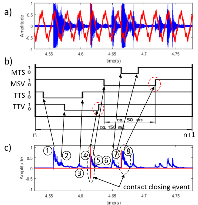
Fig. 19. (a) Originally measured vibro-acoustic signal (in blue) and arcing signal (in red) acquired from a column type OLTC when it moves from the tap position n to the tap position n + 1 ; (b) timing diagram of OLTC contacts; and (c) results of Savitzky-Golay filters for processing vibro-acoustic and arcing signals (red impulses are the arcing signals extracted and blue signals are the vibro-acoustic signals smoothed by Savitzky-Golay filters). MTS – main switch, MSV – main vacuum switch, TTS – transition switch, TTV – transition vacuum switch.
