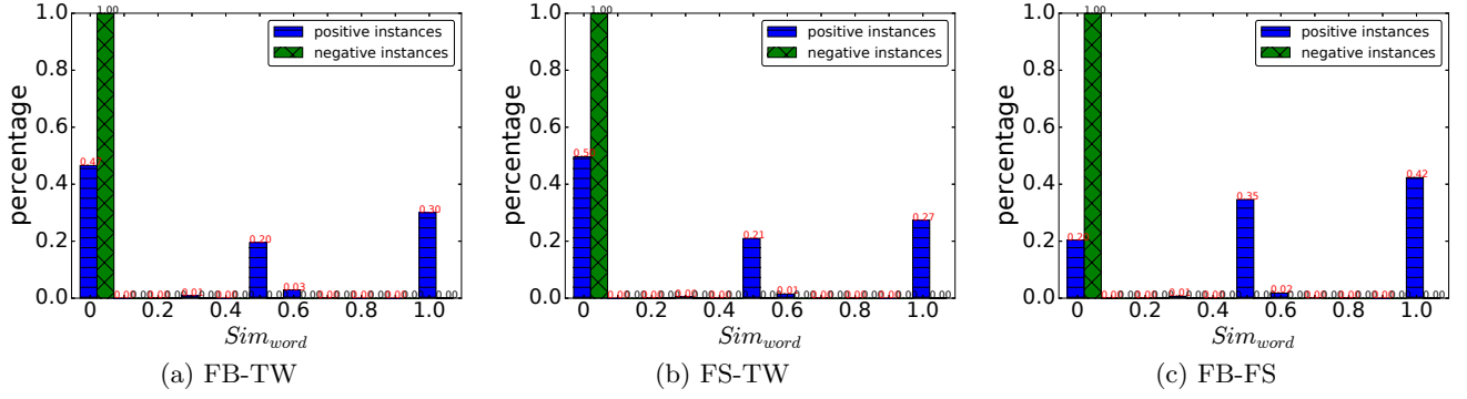
Figure 6: Distribution of Sim_{word} on three Datasets
