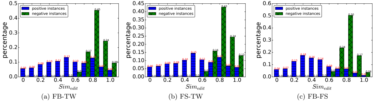
Figure 7: Distribution of Sim_{edit} on three Datasets
