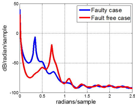
Figure 3: PSD of the main shaft axial acceleration.
