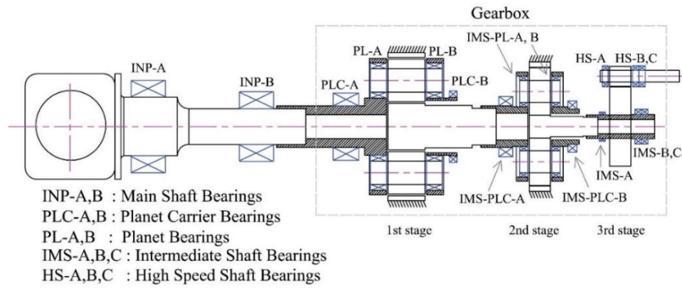
Figure 1: 5 MW reference gearbox layout [30].
