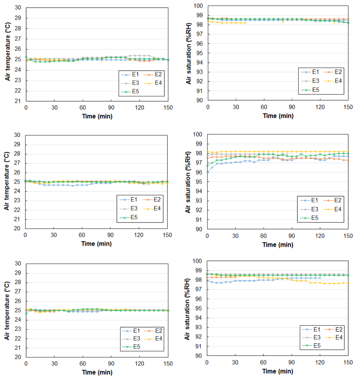
Figure C.4 Evolution of the air temperature and saturation throughout the experiments with air injection on L-arginine solutions. Top: 1100 µl/min; Middle: 1500 µl/min; Bottom: 2100 µl/min. E1-E5 correspond to 5 repetitions at the same conditions. Each of these repetitions contains up to 16 parallel samples.
