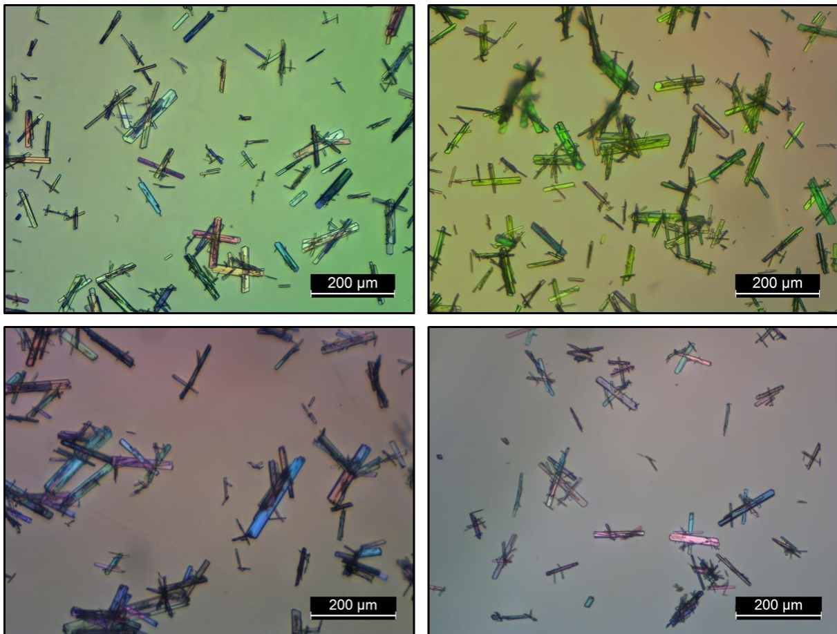
Figure 6.7 Microscope pictures of the crystallization magma from runs A1.3 (top left), A3 (top right), A4 (bottom left) and the second attempt at A6 (bottom right).
