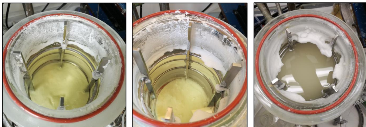
Figure 6.5 Crust formation at the top of the MSMPR crystallizer. Left: end of experiment A3 Middle: end of experiment A5. Right: end of the first attempt at experiment A6. None of the other experiments in this work presented this phenomenon.
