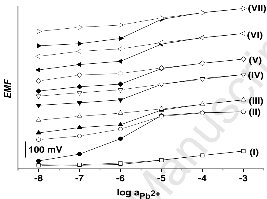
Fig. 6. Potentiometric response of \text{Pb}^{2+} -ISEs measured for increasing \text{Pb}^{2+} concentrations (filled symbols), followed by decreasing \text{Pb}^{2+} concentrations (open symbols) after application of different conditioning solutions: conditioned in 10^{-3} \text{ mol dm}^{-3} \text{ Pb}^{2+} for 24 h (I) followed by conditioning in 0.01 \text{ mol dm}^{-3} \text{ PBS} for 3 h (II) and followed by conditioning for 3 h in 0.01 \text{ mol dm}^{-3} \text{ PBS} containing 0.1 (III), 0.25 (IV), 0.5 (V), 1 (VI) and 2 (VII) \text{mg ml}^{-1} \text{ BSA} .
