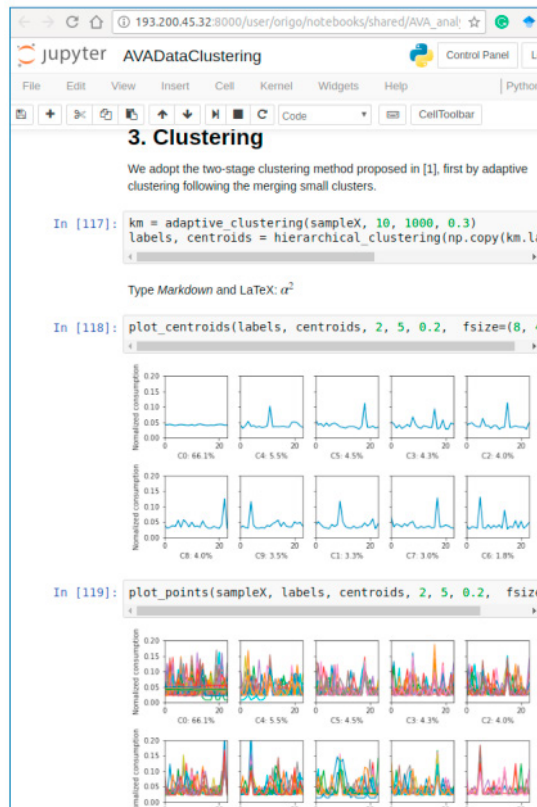
Figure 2 Data analysis by Jupyterhub
