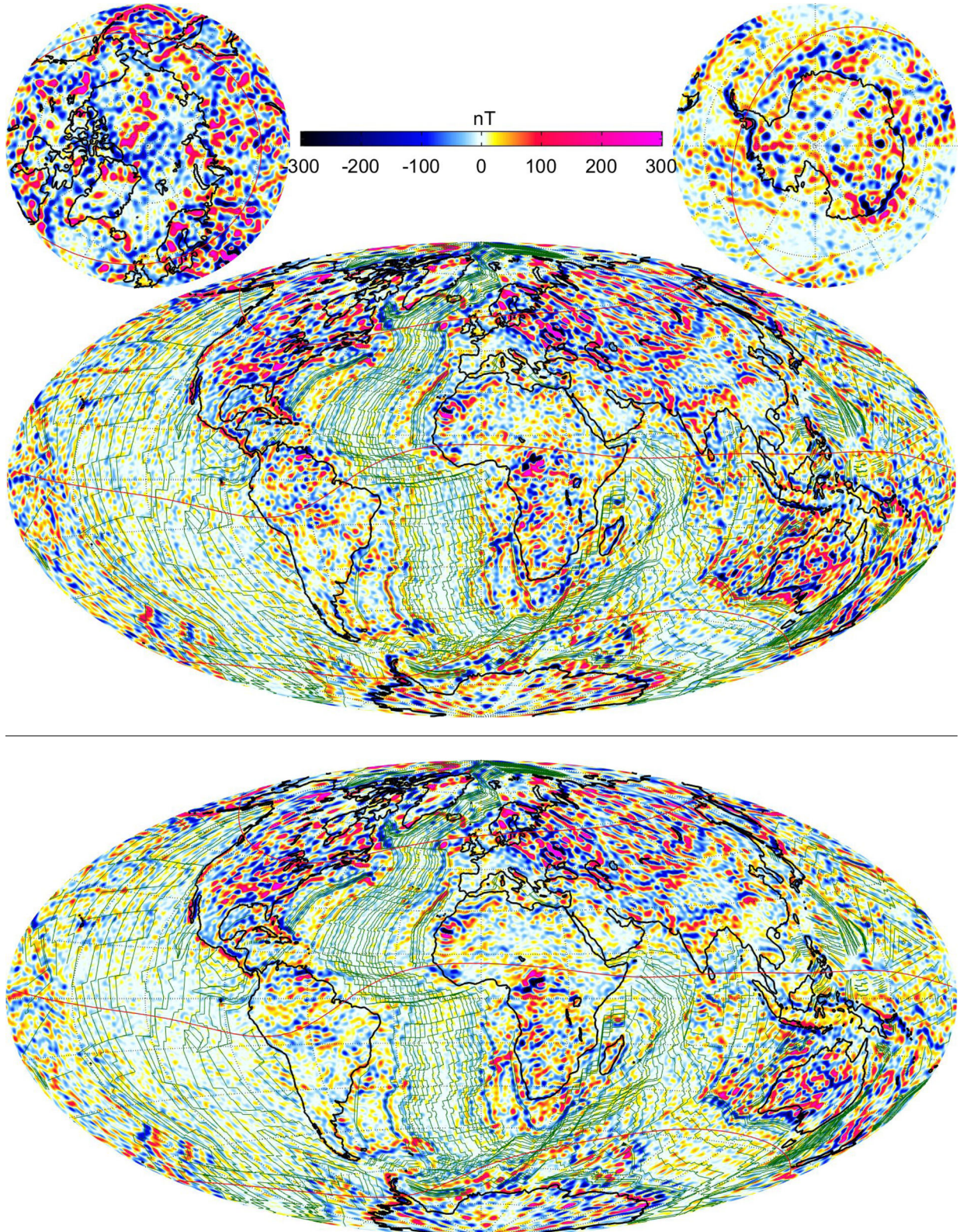
Figure 7. Maps of the lithospheric field vertical component Z (top) and of scalar anomaly F (bottom) at Earth's surface (ellipsoid) from the LCS-1 model, for spherical harmonic degrees n = 16 – 185 . Red curves represent QD latitudes of \pm 55^\circ , respectively 0^\circ , while green curves show isochrones.
