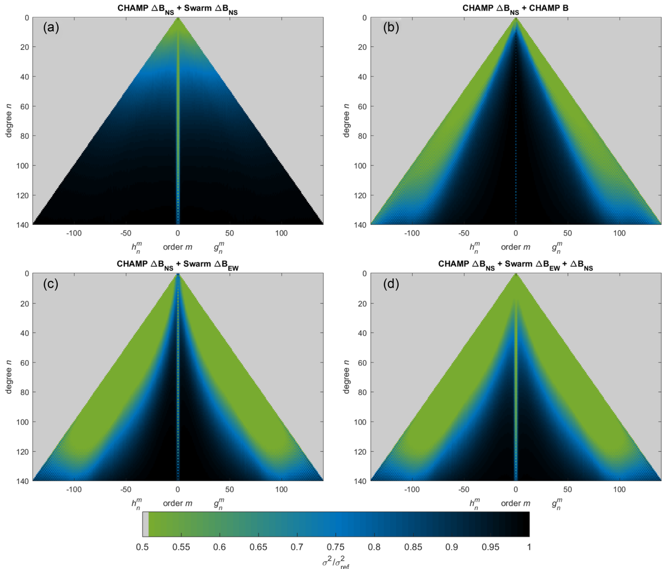
Figure 6. Variance ratio for models estimated from combined CHAMP + Swarm data sets, compared to the CHAMP-only model of Fig. 5b). Green corresponds to potential model improvement (i.e. reduction of variance), while black corresponds to no improvement.
