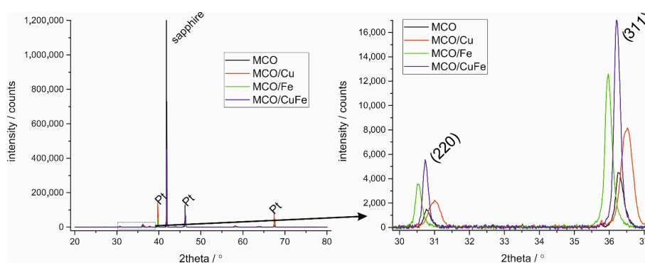
Figure 7. XRD at RT after exposure to 800 °C.
