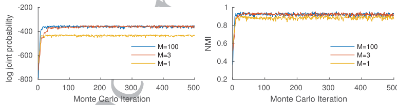
(e) The log joint probability over (f) The NMI over MCMC iterations. MCMC iterations.
