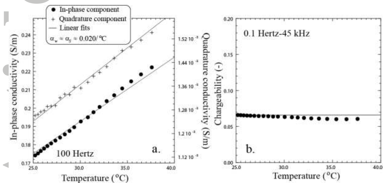
Figure 22. Influence of the temperature. a. Influence of the temperature on the magnitude of the in-phase and quadrature components of the complex conductivity. b. Influence of the temperature on the chargeability. As predicted by the dynamic Stern layer model, the chargeability is nearly temperature independent.
