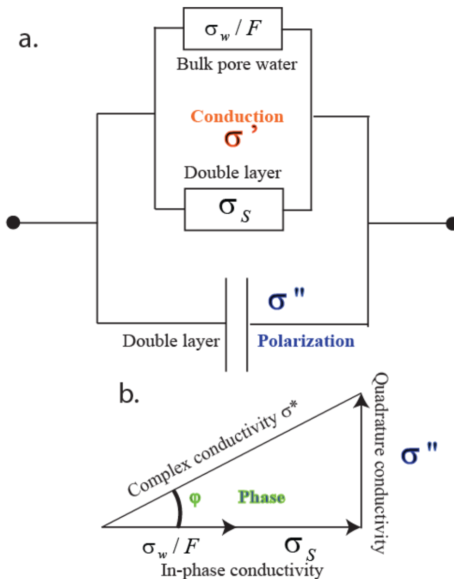
Figure 4. First-order approximation of the equivalent circuit of a soil at high frequencies. a. Equivalent circuit. Conduction associated with the electromigration of the charge carriers comprises two contributions, one associated with the bulk pore water and the other with conduction in the electrical double layer (including the Stern and diffuse layers). The capacitance corresponds to the polarization of the Stern layer coating the surface of the grains (Figure 1). b. Complex conductivity representation. The complex conductivity \sigma^* is characterized by an in-phase component and a quadrature component. The tangent of the phase angle \varphi represents the ratio between polarization (described by the quadrature conductivity \sigma'' or the normalized chargeability M_n ) and conduction described by the in-phase conductivity \sigma' . This in-phase conductivity is itself the sum of two contributions, a bulk conductivity (given by the conductivity of the pore water \sigma_w divided by the formation factor F ) and a surface conductivity \sigma_s .
