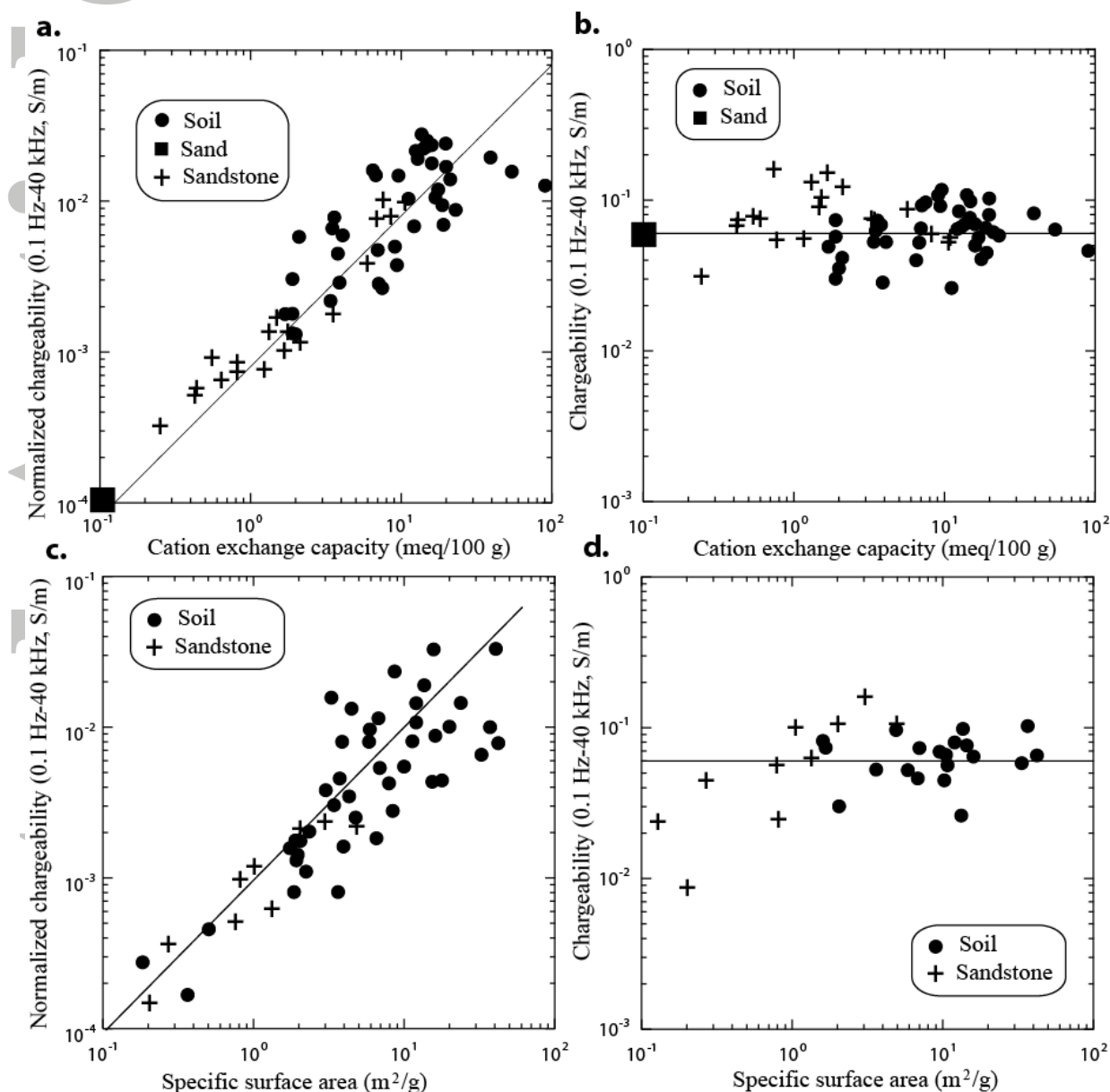
Figure 21. Linear relationship between the normalized chargeability (between 0.1 Hertz and 40 kHz) and the chargeability for the soil samples at 0.03 \text{ S m}^{-1} (NaCl, 25^\circ\text{C} ) versus either the cation exchange capacity and the specific surface area. a. Normalized chargeability versus CEC. b. Chargeability versus CEC. For a) and b) the sandstone data are from Vinegar and Waxman [1984] (all samples at the lowest salinity, the normalized chargeability are obtained using his quadrature conductivity data at 0.1 \text{ S m}^{-1} using \alpha = 8 ). c. Normalized chargeability versus specific surface area. d. Chargeability versus specific surface area. For b) and c), the sandstone data are from Börner [1992] where the normalized chargeability are obtained using his quadrature conductivity data at 0.1 \text{ S m}^{-1} using \alpha = 8 .
