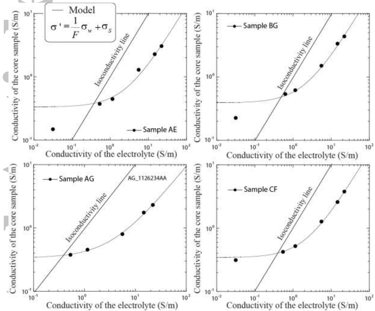
Figure 12. Conductivity of the material versus the pore water conductivity for 4 samples (AE: Dark sandy clay, AG: gray sand, CF: gray clay, BG: gray clay). We see clearly that the data exhibit an isoconductivity point (at the intersection of the two curves, one being the isoconductivity line and the other the linear conductivity model, see equations 5).
