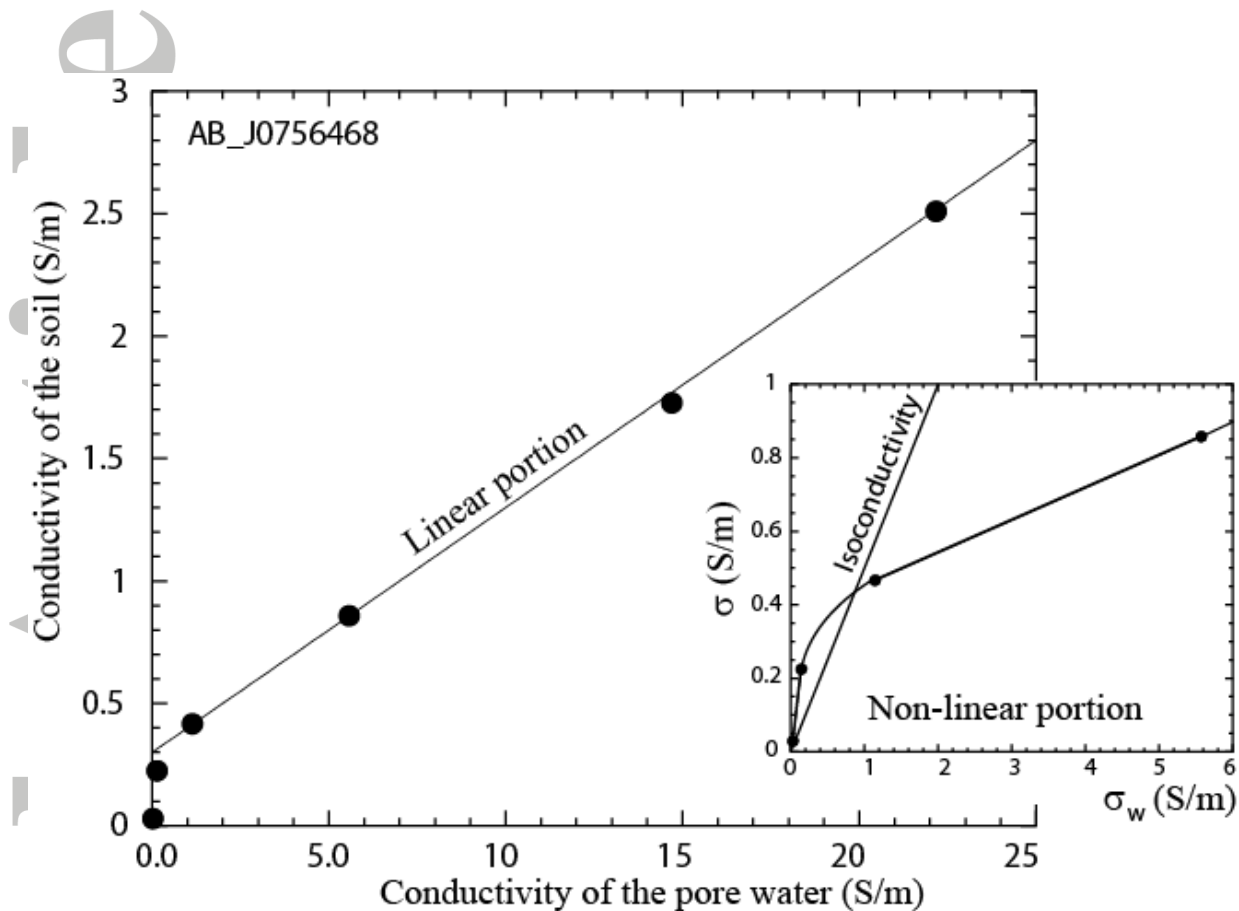
Figure 10. Conductivity versus pore water conductivity showing the linear (obeying to equation 5) and non-linear portions of the conductivity plot. The non-linear portion at low salinities is due to a change in the tortuosity of the conduction paths. The quantities \sigma and \sigma_w define the conductivity of the soil and the conductivity of the pore water.
