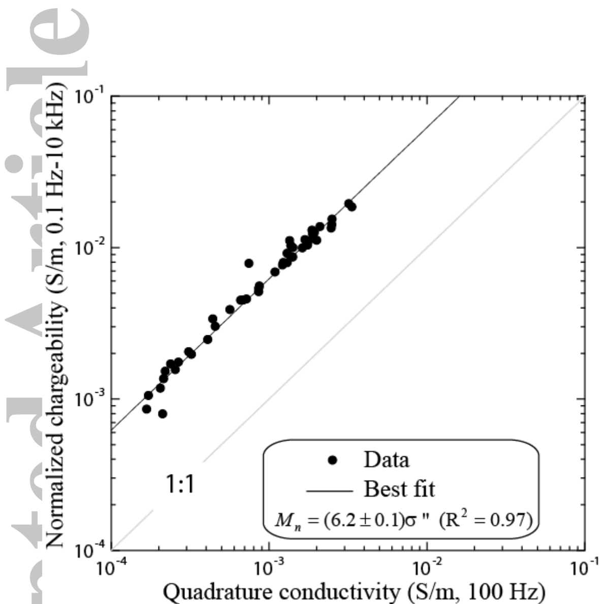
Figure 16. Relationship between the normalized chargeability and the quadrature conductivity for the low salinity dataset and the frequency range 0.1 Hertz-10 kHz. The theoretical prediction is \alpha \approx -(2/\pi)\ln D . If we assume that high and low frequencies are separated by 5 decades ( D = 10^5 ), we obtain \alpha \approx 5.9 consistent with the best fit of the data ( 6.2 \pm 0.1 ).
