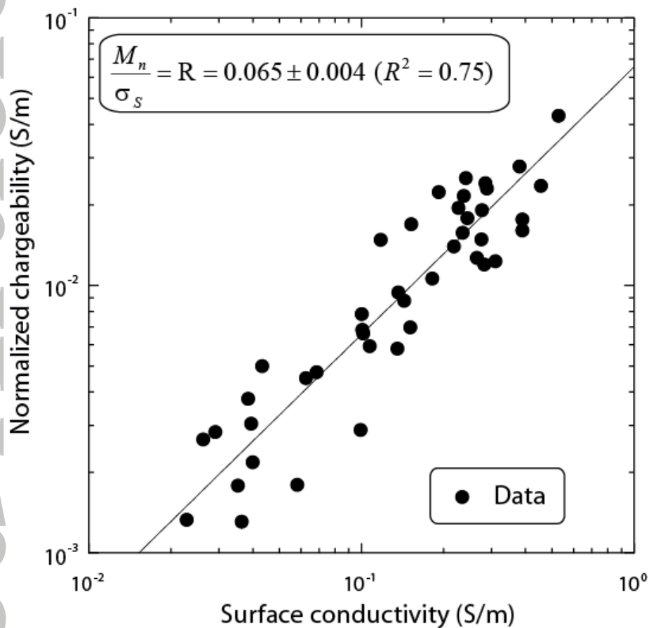
Figure 19. Linear relationship between normalized chargeability (between 0.1 Hertz and 40 kHz) and surface conductivity for the soil samples at 0.03 \text{ S m}^{-1} (NaCl, 25^\circ\text{C} ). The plain line corresponds to the best fit of the data using a linear model between the normalized chargeability and the surface conductivity.
