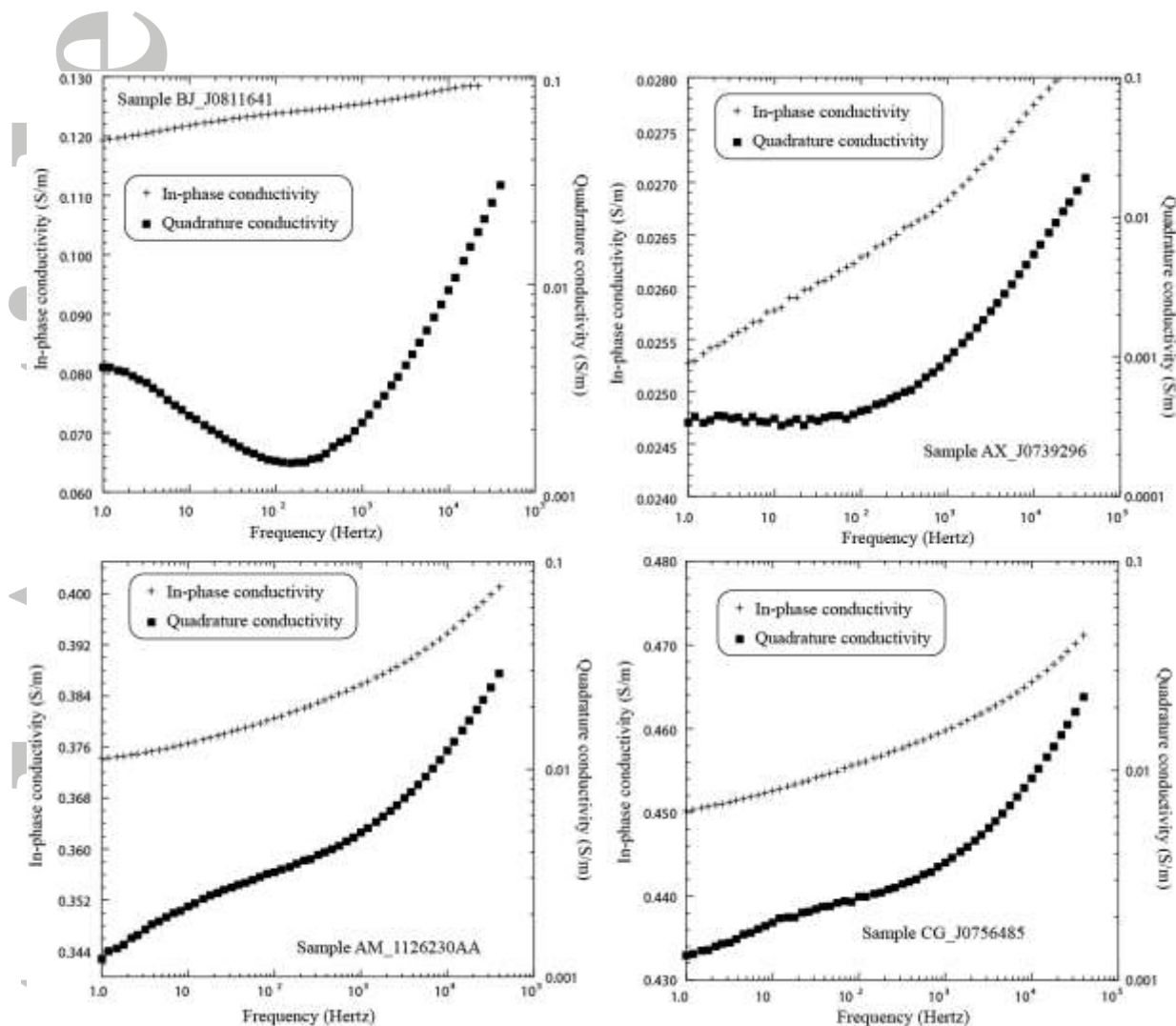
Figure 8. Complex conductivity spectrum (real/in-phase and absolute value of the imaginary/quadrature components). Sample BJ_J0811641 (Gray sandy clayey soil), sample AM-1126230AA (Gray/black clayey soil), sample AX_J0739296 (fine sand), and sample CG_J0756485 (clay). The strong increase of the quadrature conductivity above 1 kHz corresponds to dielectric phenomena including the Maxwell Wagner polarization. Spectra are reported here at the lowest salinity.
