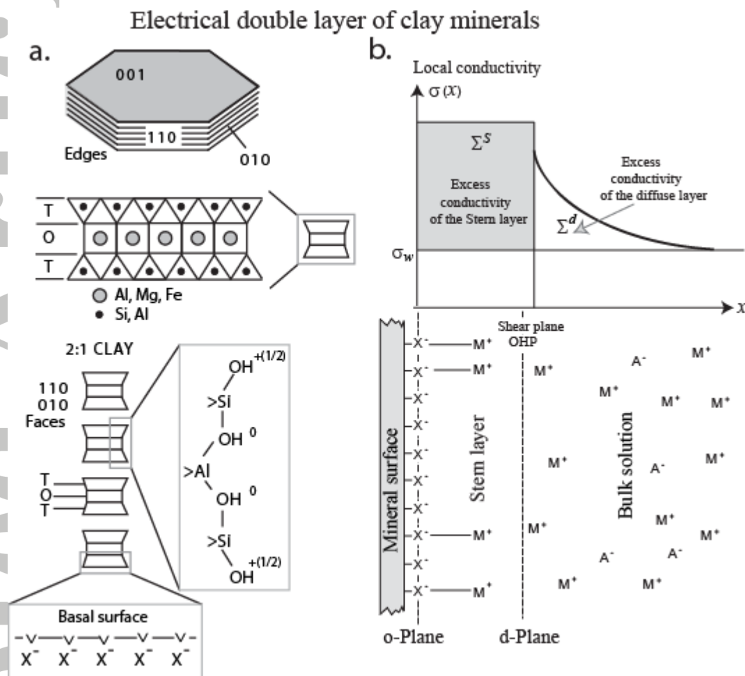
Figure 1. Nature of the electrical double layer in clay minerals. a. Clay minerals are characterized by a pH-dependent charge on the edge of their particles and, for some of them like smectite, a permanent charge associated with isomorphic substitutions in their crystalline framework. b. The effective charge density is counterbalanced by ions in the Stern and diffuse layers. This gives rise to two excess conductivities defined as the integral over the distance of the difference between the local conductivity \sigma(x) and the conductivity of the pore water \sigma_w . The surface conductivities \Sigma^S and \Sigma^d correspond to the contributions associated with the Stern and diffuse layers, respectively.
