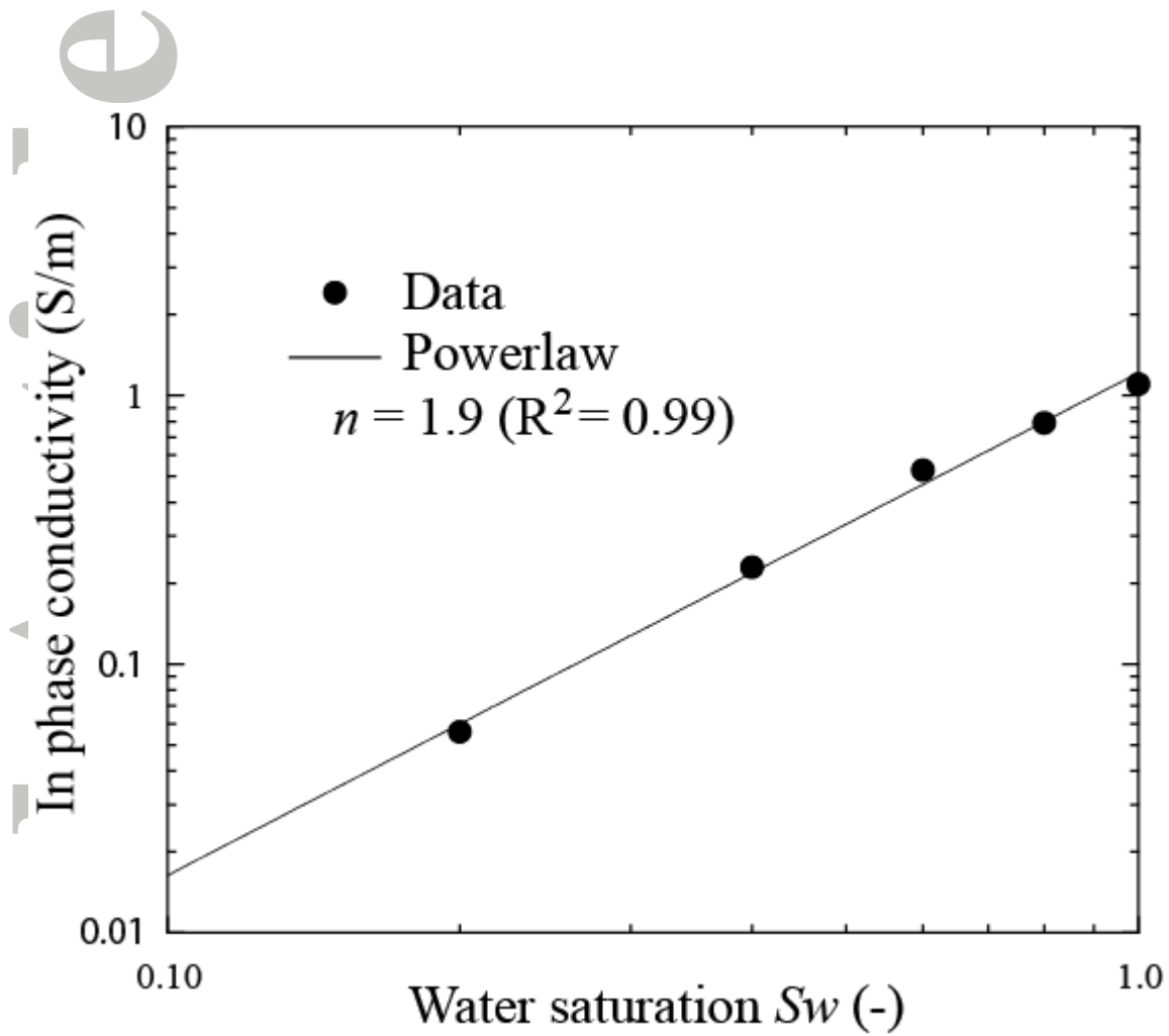
Figure 24. Saturation dependence of the in phase conductivity (1 Hertz) at high salinity (NaCl solution at 5 \text{ S m}^{-1} , sample BB, fine sand). The dependence is used to determine the second Archie's exponent n .
