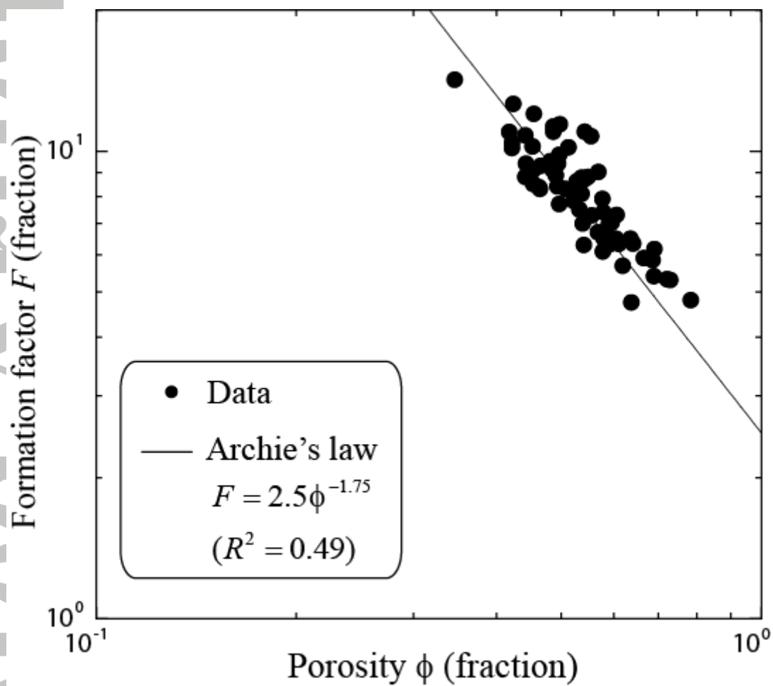
Figure 13. Relationship between the formation factor and the porosity and fit with the empirical Archie's law (peat samples excluded).
