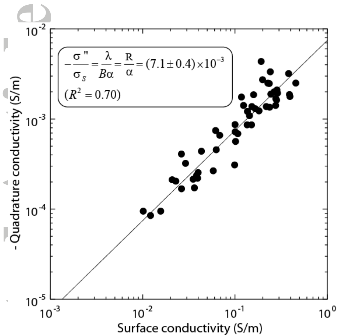
Figure 17. Direct linear relationship between quadrature conductivity and surface conductivity for the soil samples at the low pore water conductivity of 0.03 \text{ S m}^{-1} (NaCl, 25^\circ\text{C} ). Here we are below the isoconductivity point and the surface conductivity is considered to be directly equal to the in-phase conductivity. Both the in-phase and quadrature conductivity are taken at 100 Hertz. Taking \alpha = 8 , this yields R = 0.057 .
