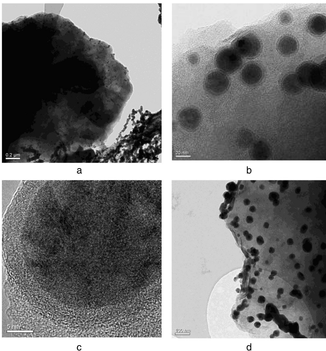
Fig. 3. HR-TEM images of: a) iron nanoparticles both in chain-like morphology and in dispersed form on the bentonite surface, b) iron nanoparticles on bentonite surface, c) the core-shell structure of iron nanoparticles, and d) iron nanoparticles on bentonite surface six months after preparation.
