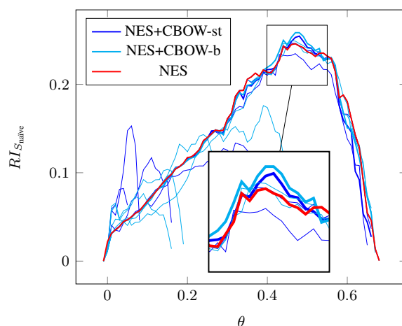
Figure 7: Rand index adjusted for S_{\text{naive}}
