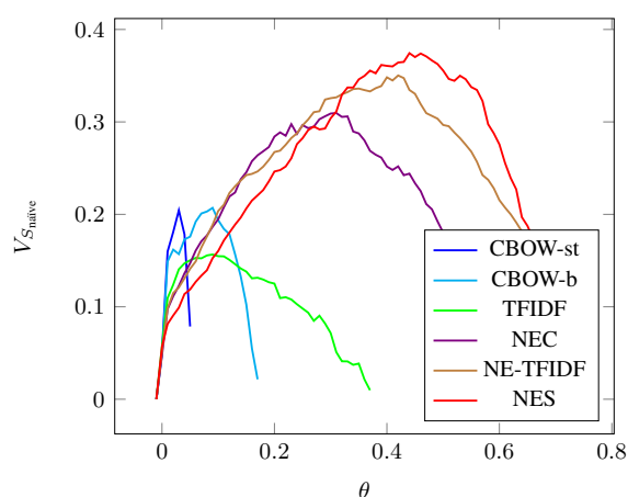
Figure 6: V Measure adjusted for S_{\text{naive}}
