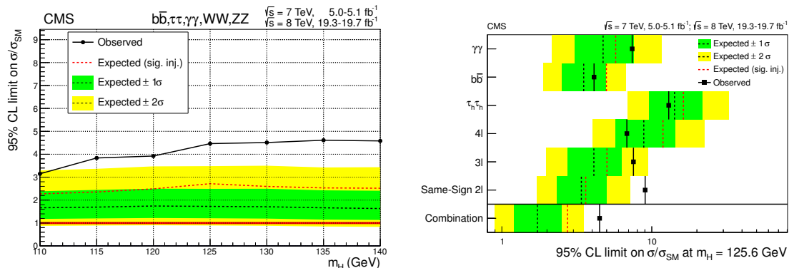
Figure 15. The 95% CL upper limits on the signal strength parameter \mu = \sigma/\sigma_{SM} . The black solid and dotted lines show the observed and background-only expected limits, respectively. The red dotted line shows the median expected limit for the SM Higgs boson with m_H = 125.6 GeV. The green and yellow areas show the 1\sigma and 2\sigma bands, respectively. Left: limits as a function of m_H for all channels combined. Right: limits for each channel at m_H = 125.6 GeV.
