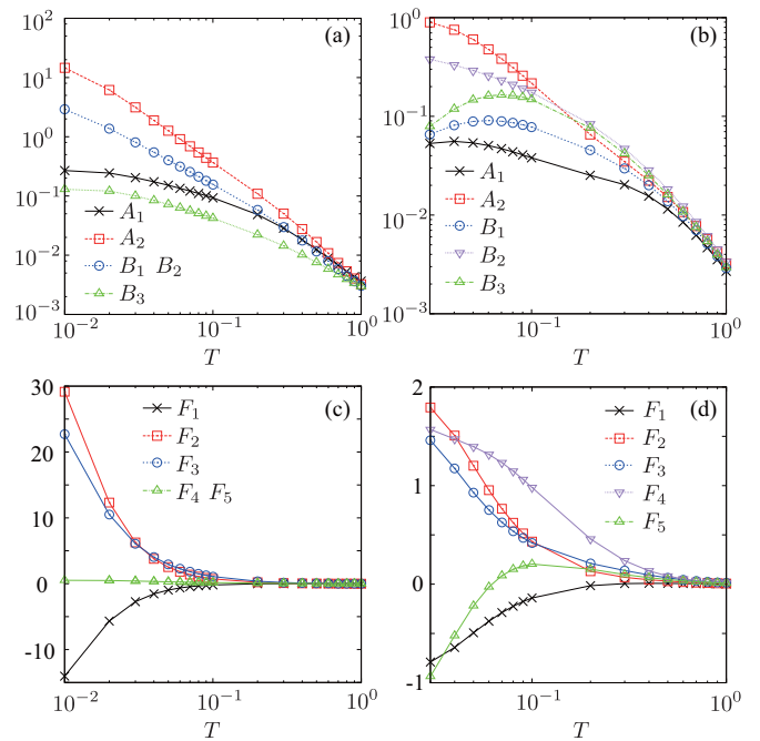
FIG. 5. (a, b) Temperature dependences of the coefficients in Eqs. (22)–(26) at (a) t_3 = -0.5 and \mu = 0.98 on the square lattice and (b) t_3 = -0.85 and \mu = -3.5 on the triangular lattice. The data are calculated for the system size N = 3600^2 and the number of Matsubara frequency 8000. (c, d) Temperature dependences of fourth-order free energy in Eqs. (17)–(21) for the same parameters in (a) and (b), respectively.
