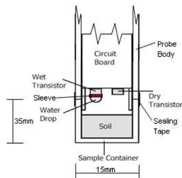
Figure 2.3 - Transistor psychrometer probe (after Bulut and Leong 2005).
