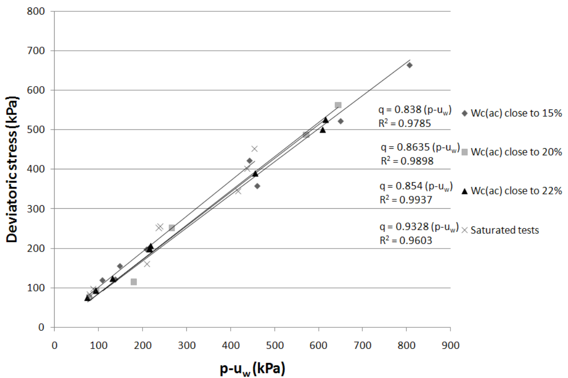
Figure 6.43 – Critical state line of the constant water tests by Wc(ac) including the saturated test series on q-(p-u w ) plane.
