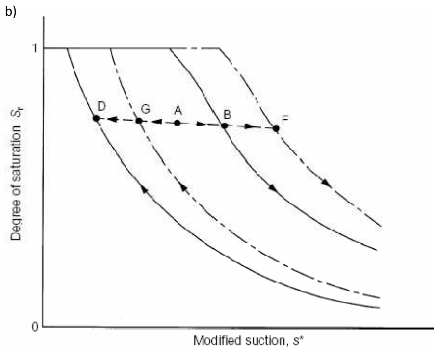
Figure 2.10 – Coupled movement of the SI and SD caused by plastic volumetric yielding:
