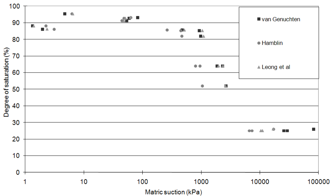
Figure 5.18 – Comparison between all matric suction SWRCs against degree of Saturation
