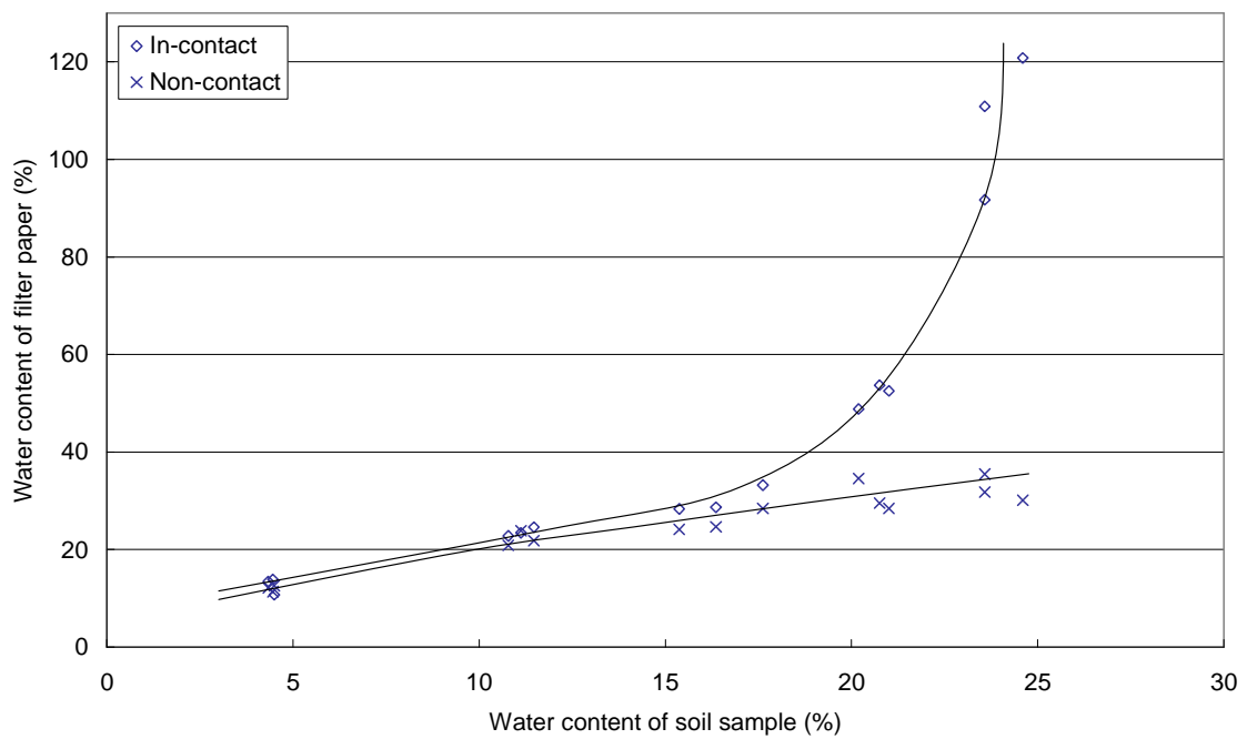
Figure 5.8 – Water contents of filter papers and corresponding soil samples at the end of equalisation period (after Noguchi, 2009).
