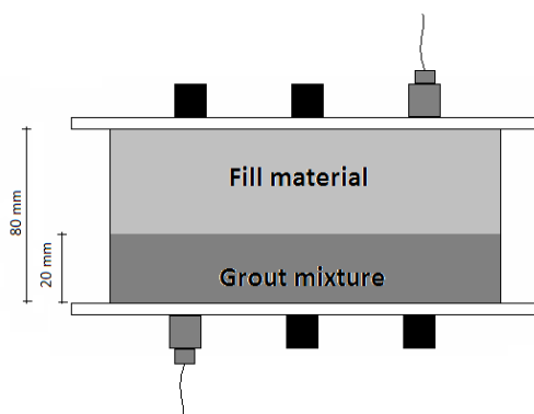
Figure 7.9 – Grout test scheme.
