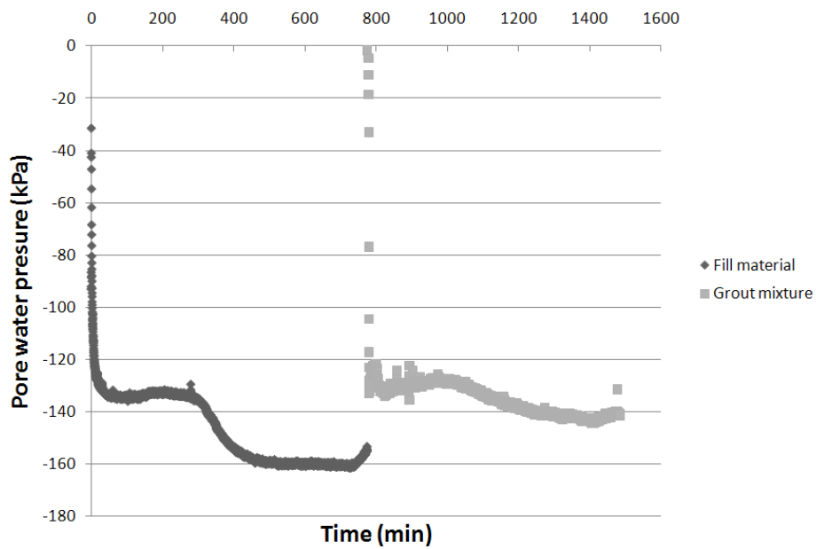
Figure 7.11 – Pore water pressure measurements on fill material and grout mixture after the first drying
