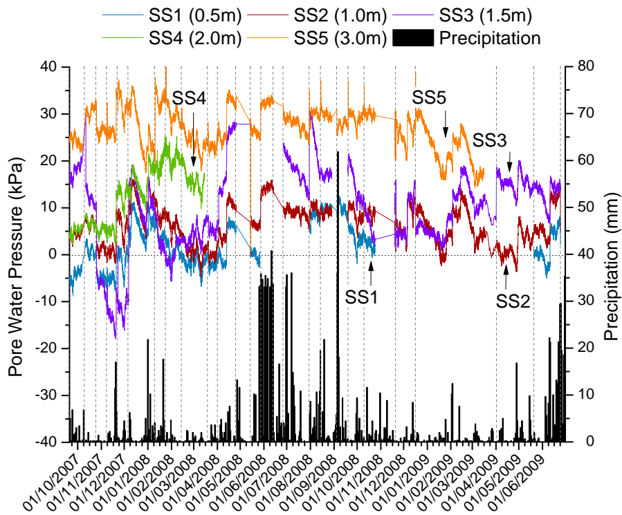
Figure 9.2 – Pore-water pressure records for the well compacted panel and rainfall. SS (X.X) indicates suction station at X.X metres depth and vertical dashed represent the reset stages.
