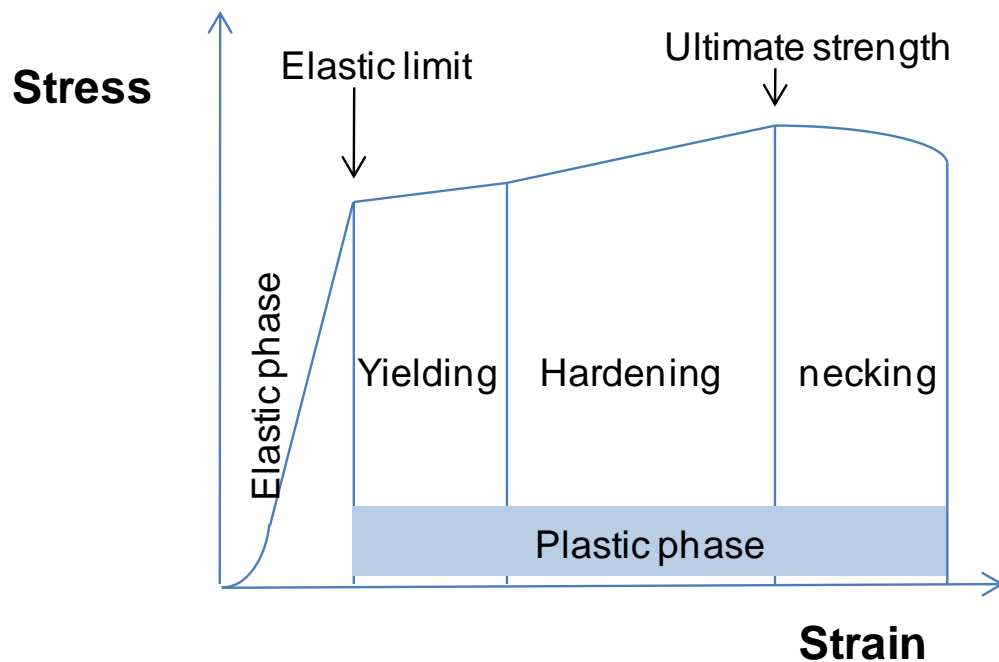
Figure 5.5 A typical stress-strain curve
