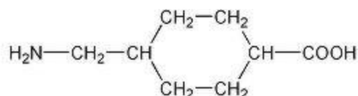
Figure 1.9 The structural formula of Tranexamic acid
