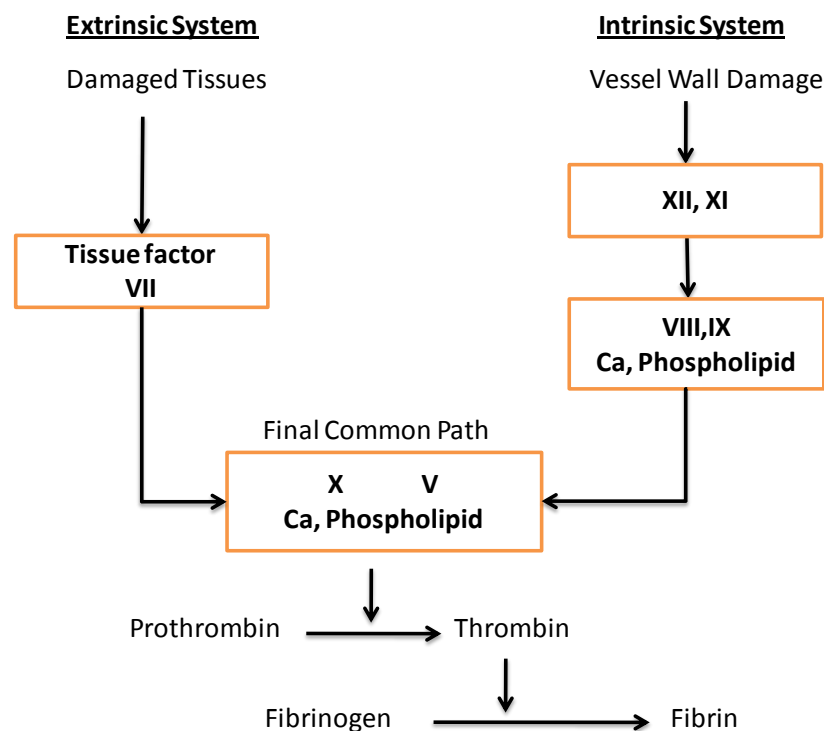
Figure 1.7 Coagulation pathways
