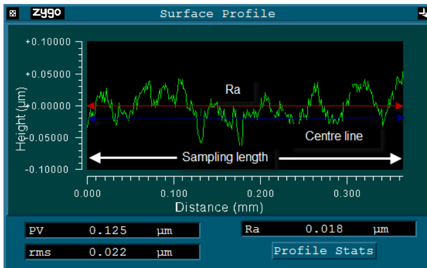
Figure 5.2 Surface roughness average (Ra)
