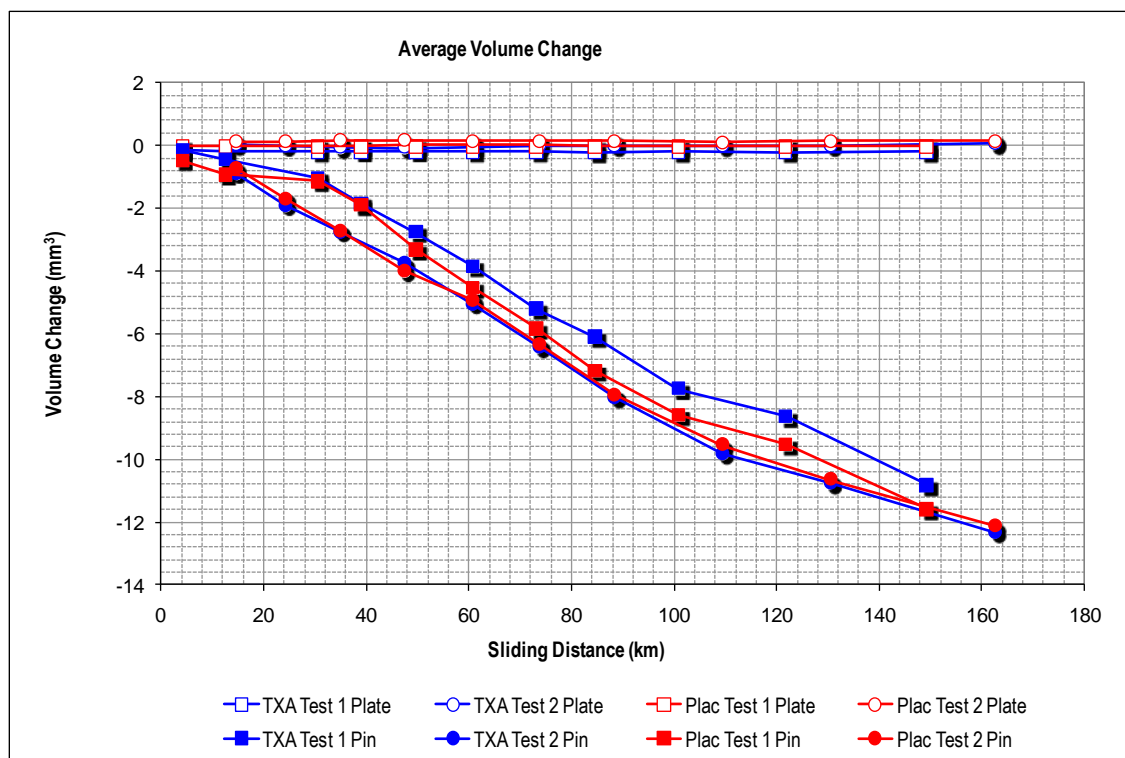
Figure 5.11 Graph of volume losses of the pins and plates plotted against sliding distance
