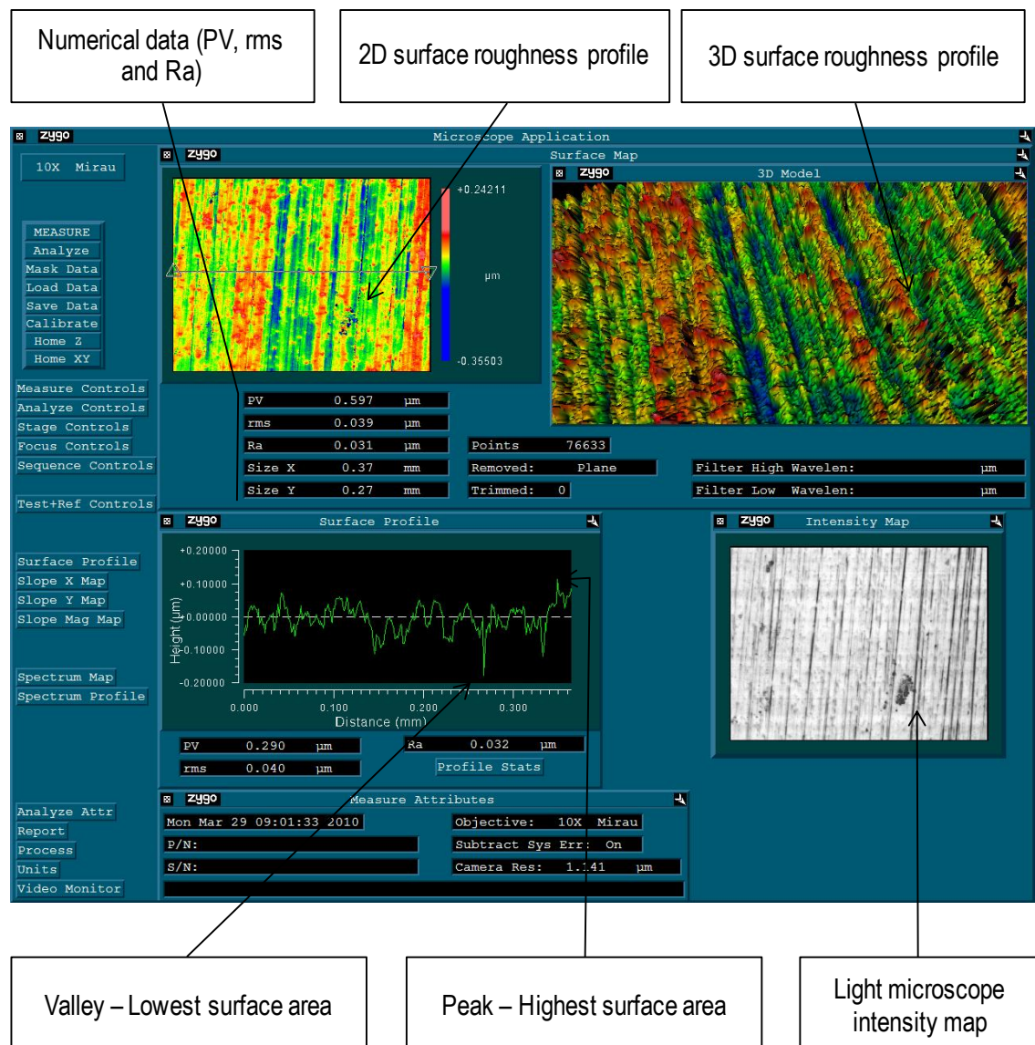
Figure 5.9 Profilometer view of surface topography of a Co-Cr plate
