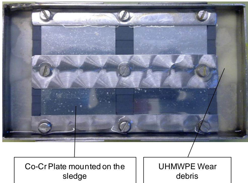
Figure 5.7 The pin-on-plate machine sledge with four Co-Cr plates mounted
