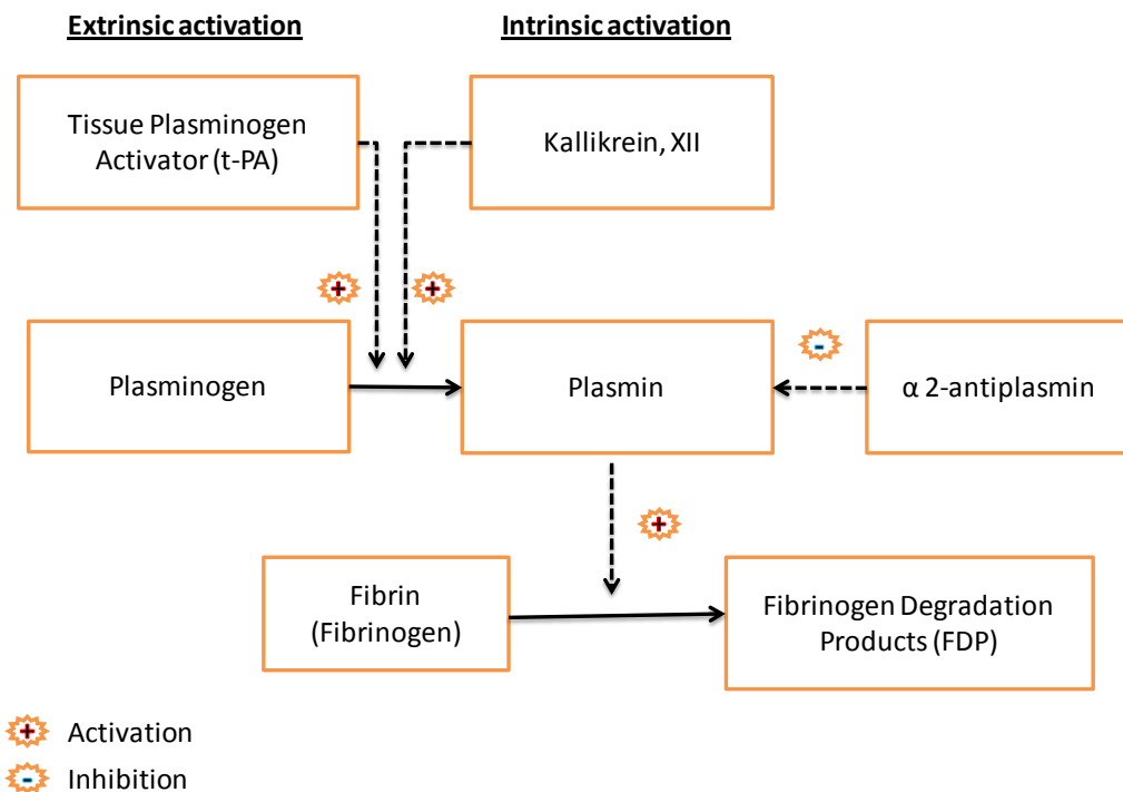
Figure 1.8 Fibrinolysis system
