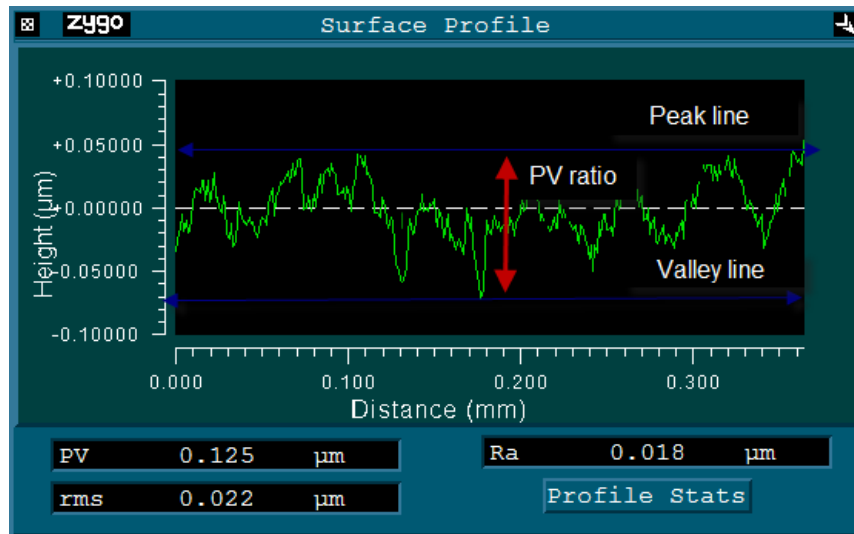
Figure 5.1 Peak-Valley ratio (PV)
