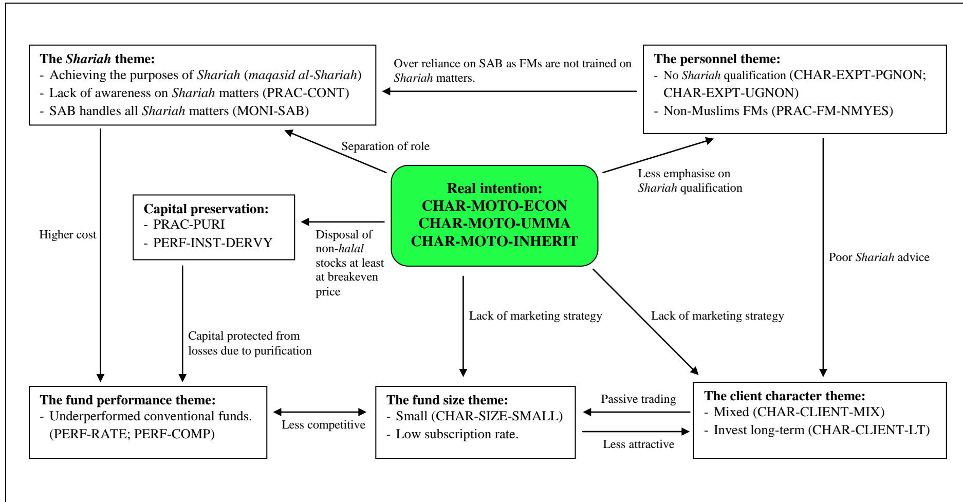
Figure 8.3: Real Intention of the Fund Management Companies in Offering Islamic Funds and Its Implications
