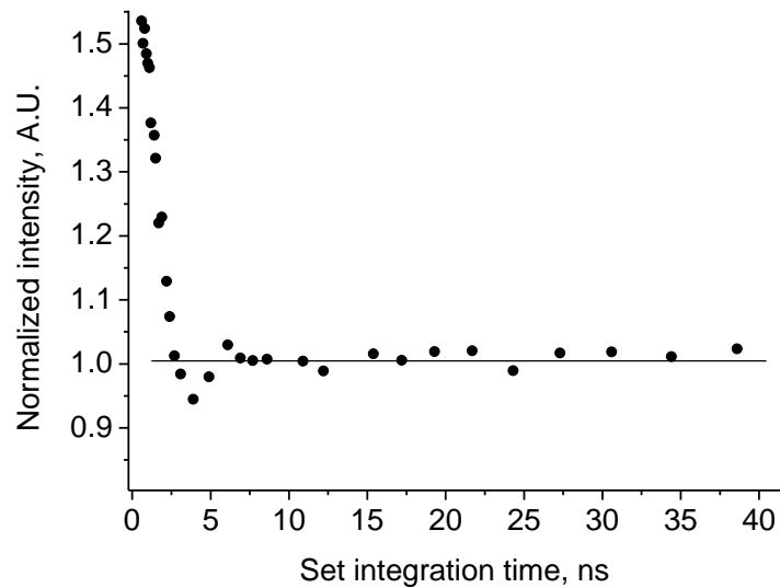
Figure 4.5 Experimental intensities of single wavelength continuous output laser diode recorded using different integration windows and divided by them. Non-linearity in region below ~ 7 ns is clearly present.
