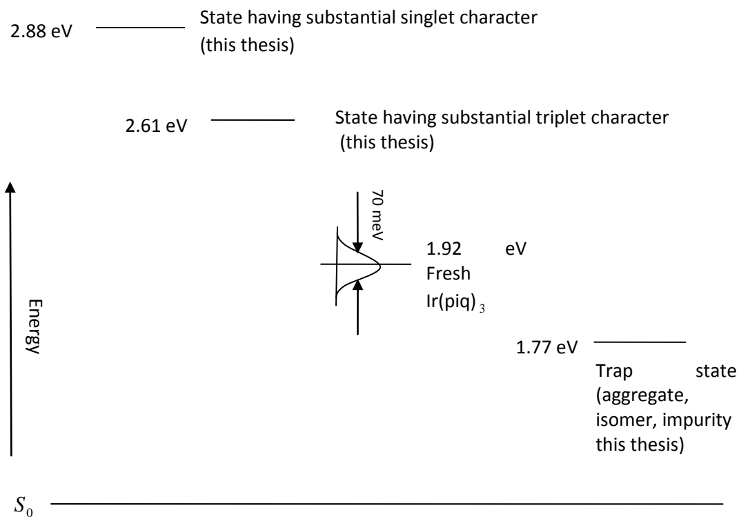
Figure 7.24 Proposed diagram of states in \text{Ir}(\text{piq})_3 films. Drawn not to scale.
