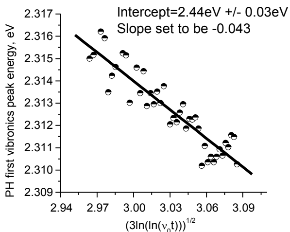
Figure 6.12 First vibronic peak of PH spectrum at 12 K plotted vs. a \ln \ln time scale. Straight line linear is fit to data, slope set to be -0.043 , intersecting ordinate axis at 2.44 \text{ eV} \pm 0.03 \text{ eV} .
