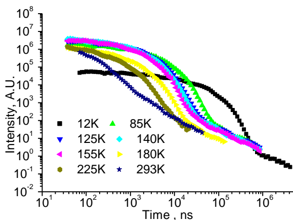
Figure 7.15 Decay curves of phosphorescence in 20 nm \text{Ir}(\text{ppy})_3 fresh film at various temperatures in log-log scale (12 K to 293 K). Excitation energy \sim 25 \mu\text{J} per pulse with 450 nm laser.
