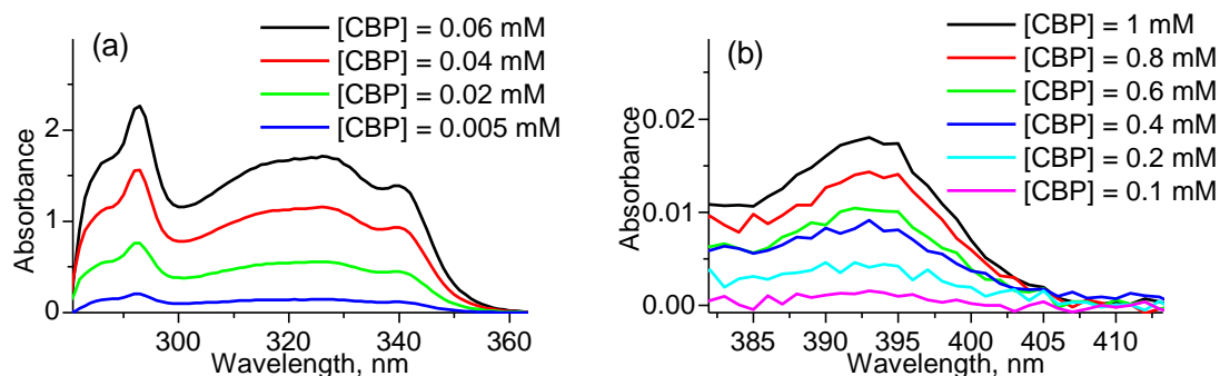
Figure 5.2 Absorption spectra of CBP in toluene of (a) low concentrated solutions in region between 280 nm and 360 nm and of (b) highly concentrated solutions in region between 382 nm and 413 nm. Square brackets around CBP is used as a sign indicating concentration.
