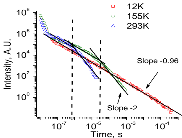
Figure 6.8 Example of how transition times t_s were determined from delayed fluorescence decay from NPB films using intersections of -0.96 and -2 curves. Linear fit with the slopes of -0.96 and -2 are shown as straight lines and indicated on the graph appropriately. Dashed lines denote the time value of intersection.
