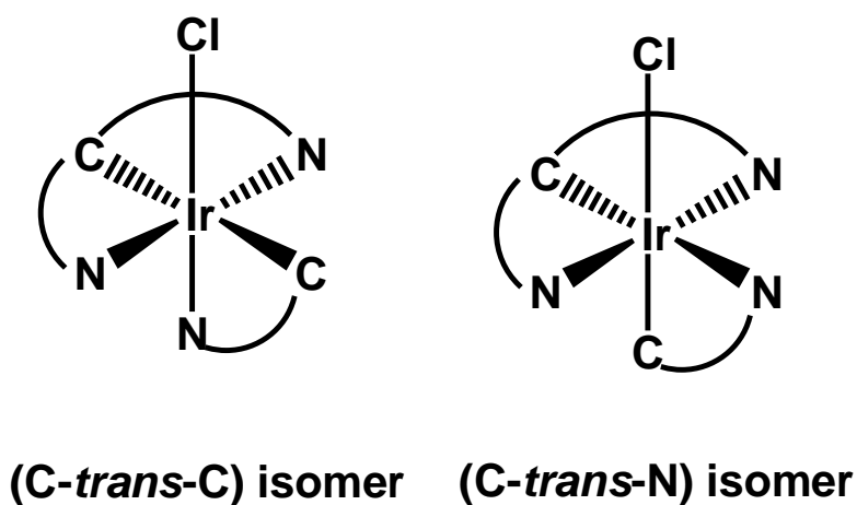
Figure 2.28: scheme of the two different isomers possible in principle for Ir(N ^C ^N )(N ^C )Cl complexes
