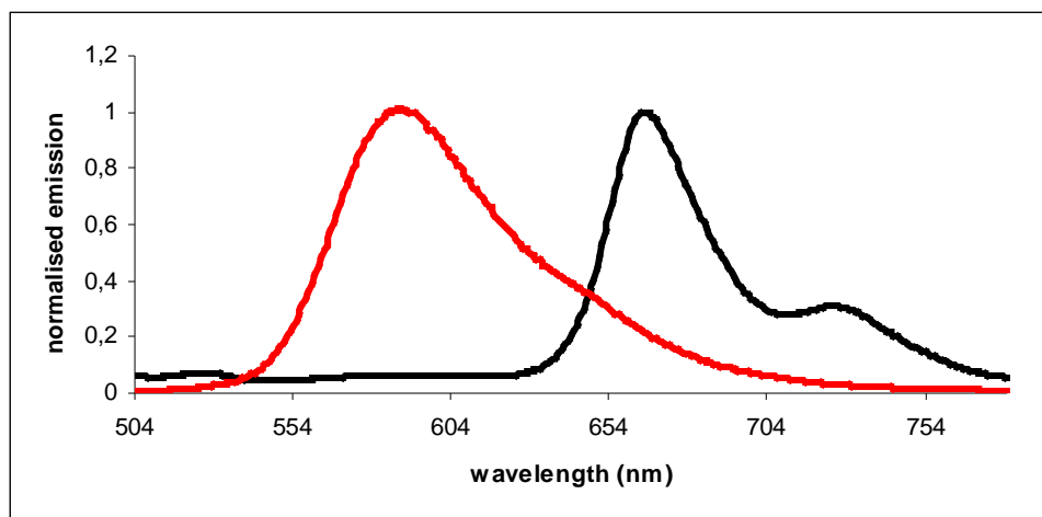
Figure 3.22: emission spectra in dichloromethane at room temperature of the complexes Ir(L3)(ppy)Cl ( 5 ) (red line) and Ir(L3)(btq)Cl ( 11 ) (black line).
