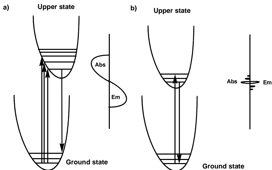
Figure 1.1: Franck-Condon effect for absorption and emission (a) for excited state and ground state having different internuclear distances and (b) for excited state and ground state of the same geometry and size.
