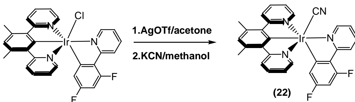
Figure 2.57: synthesis of Ir(L1)(dFppy)CN ( 22 ).
