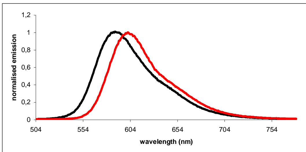
Figure 3.18: emission spectra in dichloromethane at room temperature of the complexes Ir(L3)(ppy)Cl ( 5 ) (black line), Ir(L4)(ppy)Cl ( 9 ) (red line).
