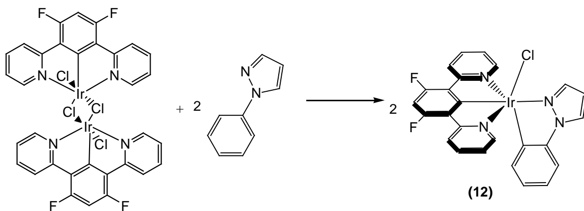
Figure 2.40: scheme for the synthesis of Ir(L2)(ppyz)Cl ( 12 ).
