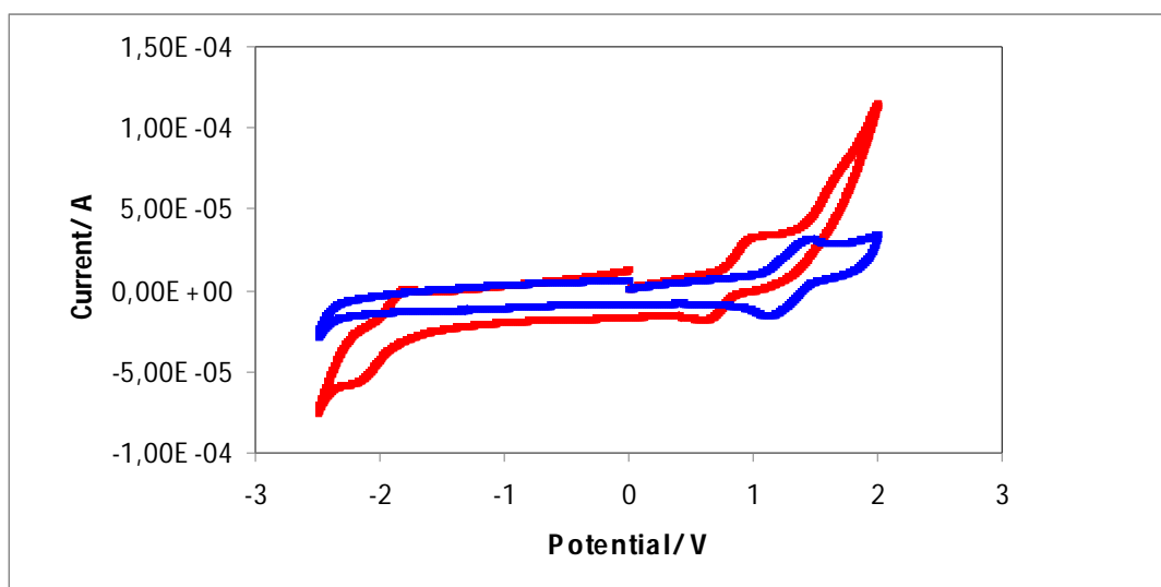
Figure 3.3: cyclic voltammetry of Ir(L3)(ppy)Cl ( 5 ) (red line) and Ir(L2)(ppy)Cl ( 4 ) (blue line), showing how the –CF 3 substituted complex is easier to oxidise than the –F substituted complex.
