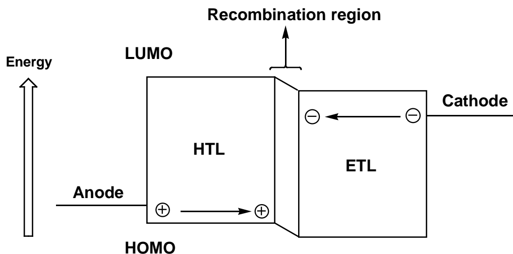
Figure 1.30: schematic recombination process in the Energy level diagram of a two-layer OLED.
