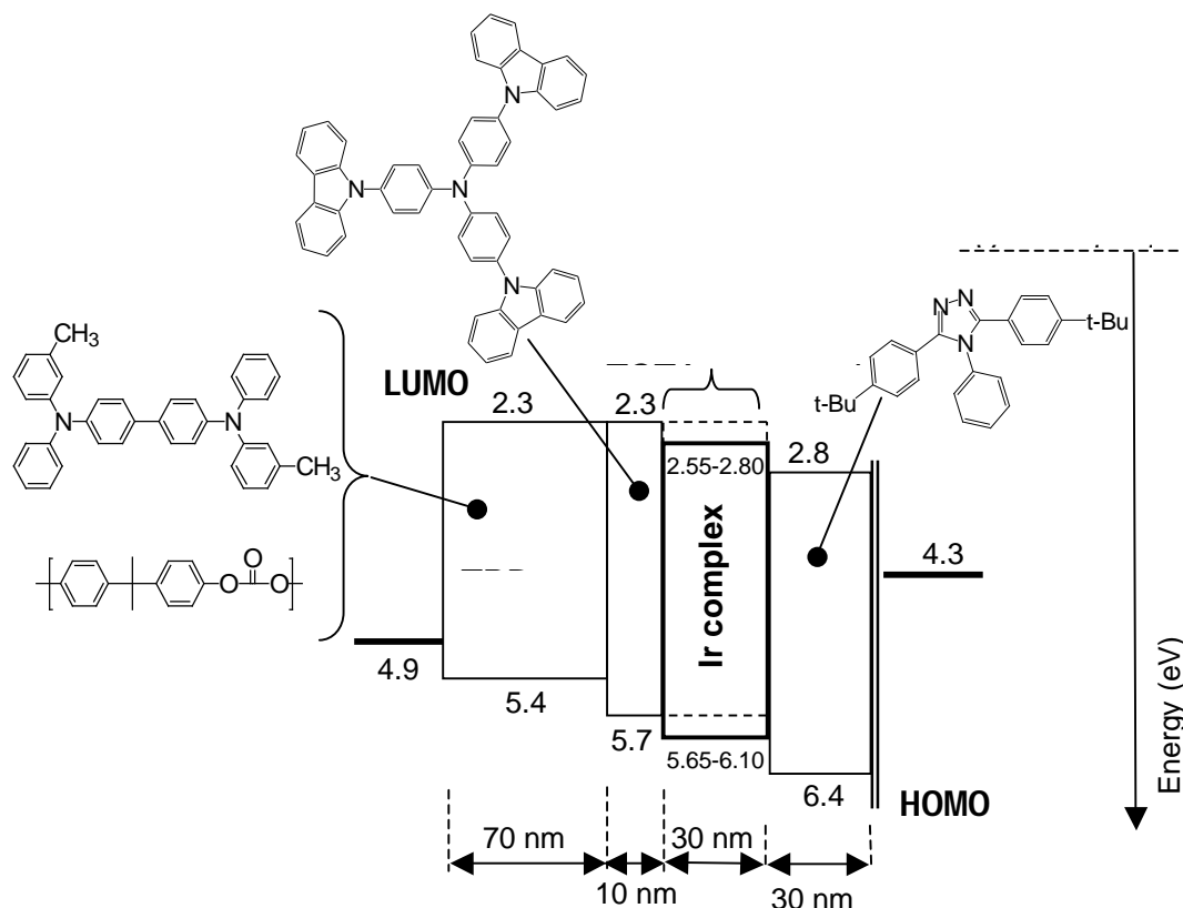
Figure 3.7 (219) : composition of the devices doped with Ir(N ^C^N )(N ^C )Cl complexes
