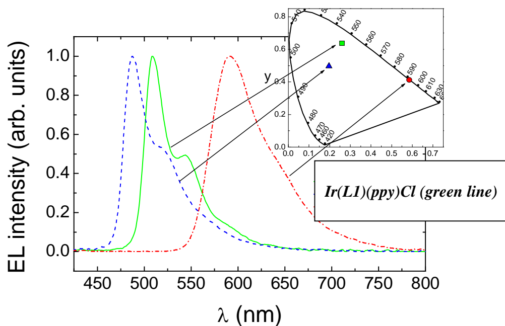
Figure 3.9: EL spectra and CIE diagram for the complexes of series 1.
