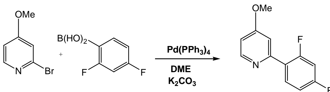
Figure 2.21: scheme for the synthesis of 2-(2,4-difluorophenyl)-4-methoxypyridine
