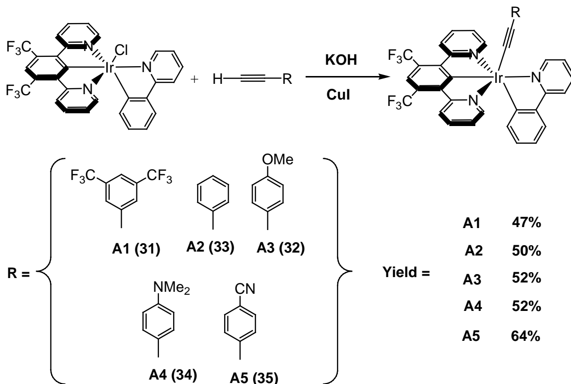
Figure 2.61: scheme for the synthesis of Ir(L3)(ppy)(acetylide) based complexes.
