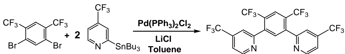
Figure 2.13: synthesis of HL4 via Stille's cross-coupling.
