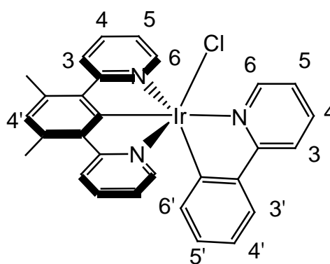
Figure 2.25 (210) : structure of Ir(L1)(ppy)Cl previously synthesised within the research group
