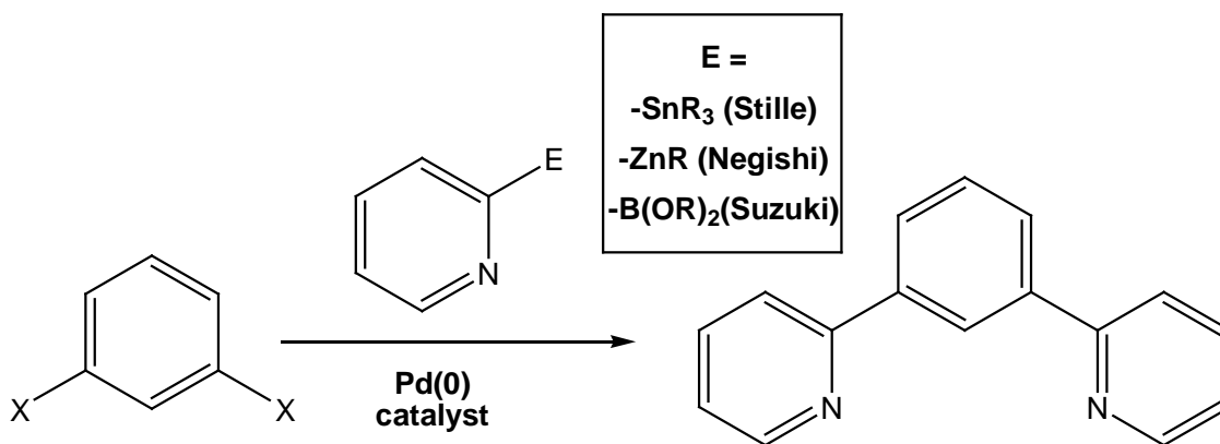
Figure 2.7 (109) : summary of the synthetic pathways leading to formation of bipyridyl ligands, Stille's method ( \text{E} = -\text{SnR}_3 precursor), Negishi's method ( \text{E} = -\text{ZnR} precursor) and Suzuki's method ( \text{E} = -\text{B(OR)}_2 ).
