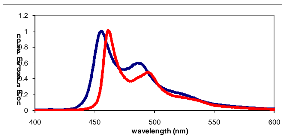
Figure 3.25: emission spectra in dichloromethane at room temperature of the complexes Ir( L2 )(dFppy)CN ( 23 ) (red line), Ir( L5 )(dFppy)CN (blue line)
