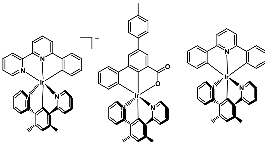
Figure 2.43 (106) : examples of \text{Ir}(\text{N}^{\wedge}\text{C}^{\wedge}\text{N})(\text{C}^{\wedge}\text{N}^{\wedge}\text{N}) , \text{Ir}(\text{N}^{\wedge}\text{C}^{\wedge}\text{N})(\text{C}^{\wedge}\text{N}^{\wedge}\text{C}) and \text{Ir}(\text{N}^{\wedge}\text{C}^{\wedge}\text{N})(\text{O}^{\wedge}\text{N}^{\wedge}\text{C}) previously synthesised by the research group
