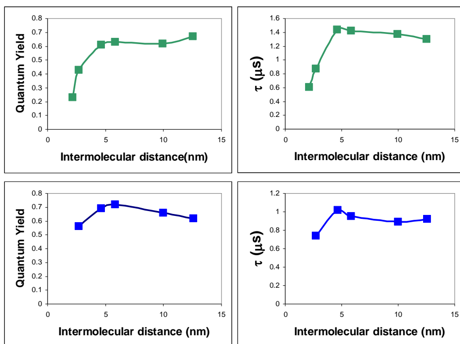
Figure 3.12: Quantum yields and lifetimes plotted against the estimated average intermolecular distance for Ir(L1)(dFppy)Cl ( 1 ) (green plot) and Ir(L2)(dFppy)Cl ( 2 ) (blue plot)
