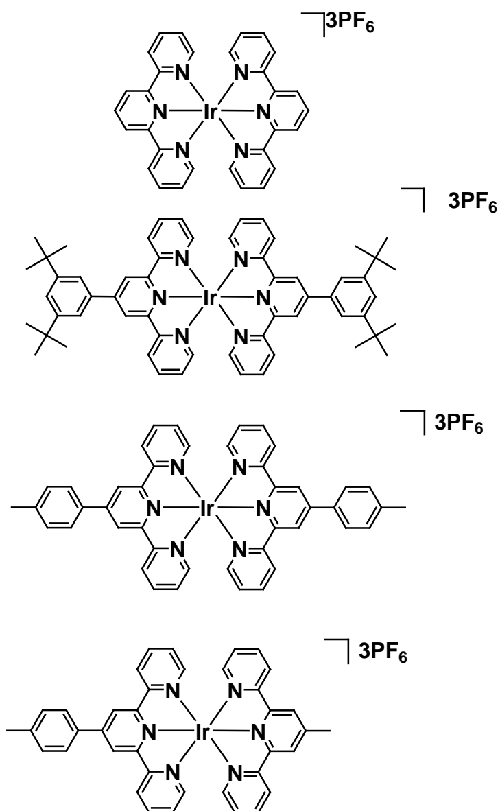
Figure 1.13 (86) : Examples of [(IrLL')_3]^{3+} complexes synthesised by Sauvage et al.
