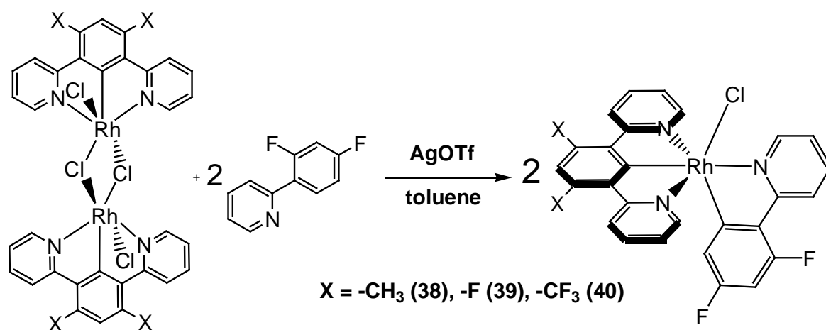
Figure 2.64: synthesis of \text{Rh}(\text{N}^{\wedge}\text{C}^{\wedge}\text{N})(\text{N}^{\wedge}\text{C})\text{Cl} , where X = -\text{CH}_3 , -\text{F} or -\text{CF}_3
