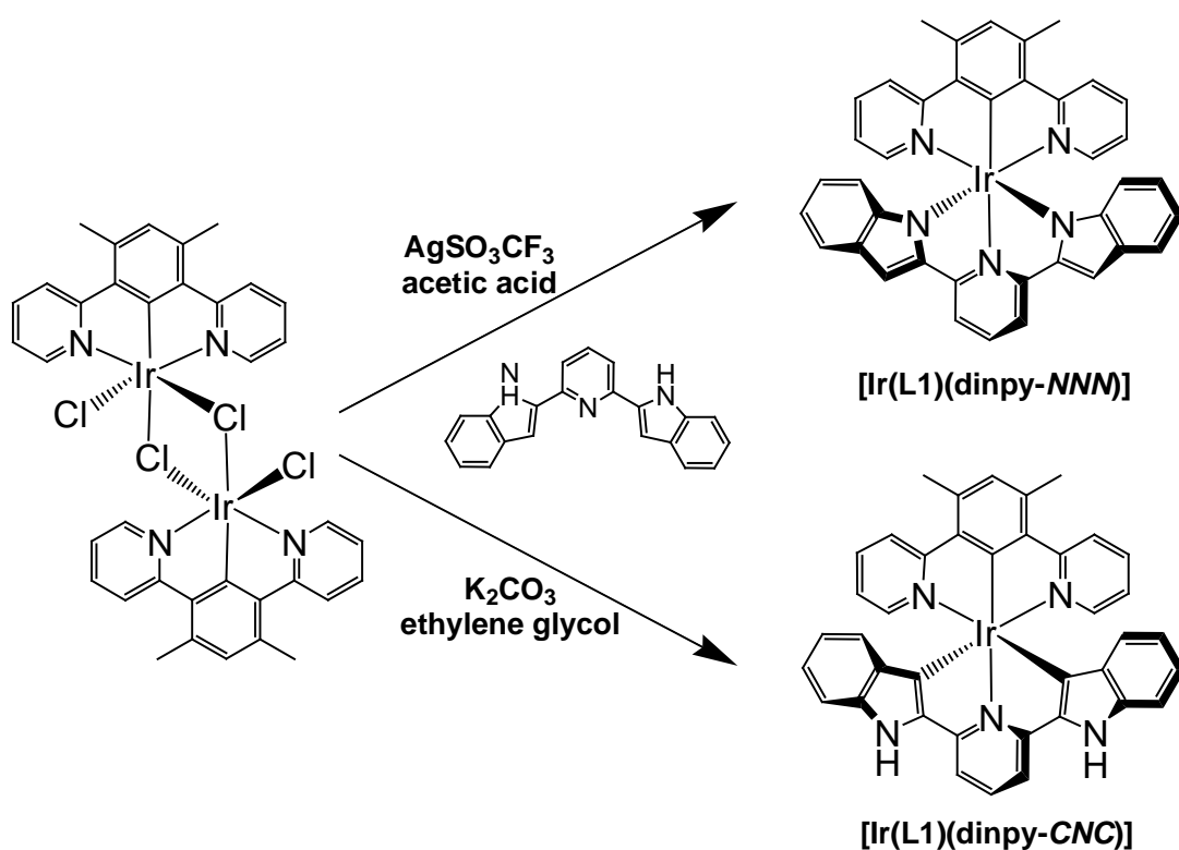
Figure 2.46 (24) : scheme for the synthesis of [\text{Ir}(\text{dpdmb})(\text{dinpy-NNN})] and [\text{Ir}(\text{dpdmb})(\text{dinpy-CNC})]
