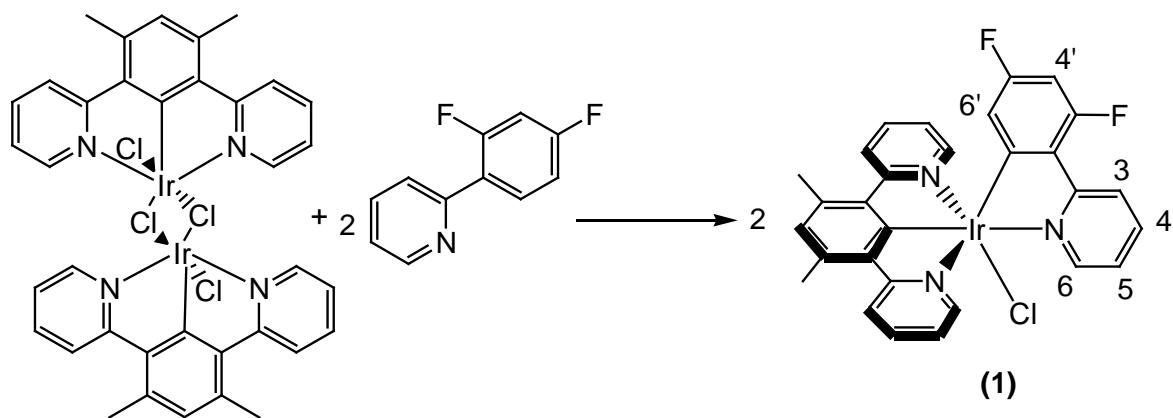
Figure 2.26: scheme for the synthesis of Ir(L1)(dFppy)Cl ( 1 ) and the atom numbering system for assignment of NMR
