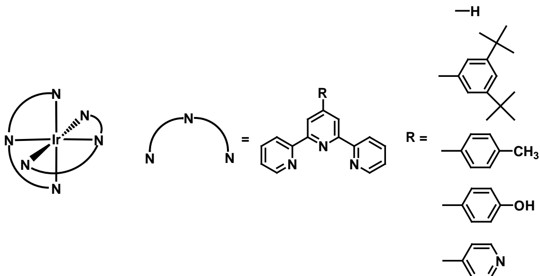
Fig. 1.12 (66) Representation of bis-terpyridine complexes.
