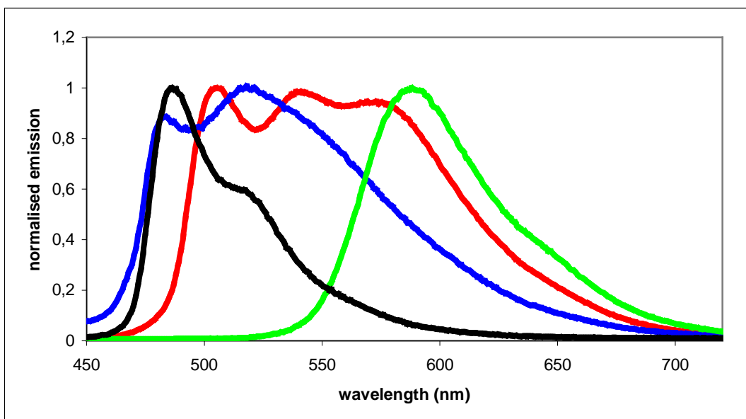
Figure 3.32: normalised emission spectra of [\text{Ir}(\mathbf{L3})(\text{bpy})\text{Cl}]^+ ( 13 ) (red line) and [\text{Ir}(\mathbf{L2})(\text{bpy})\text{Cl}]^+ ( 14 ) (blue line) in dichloromethane at room temperature, each compared with \text{Ir}(\mathbf{L3})(\text{ppy})\text{Cl} ( 5 ) (green line) and \text{Ir}(\mathbf{L2})(\text{ppy})\text{Cl} ( 4 ) (black line).
