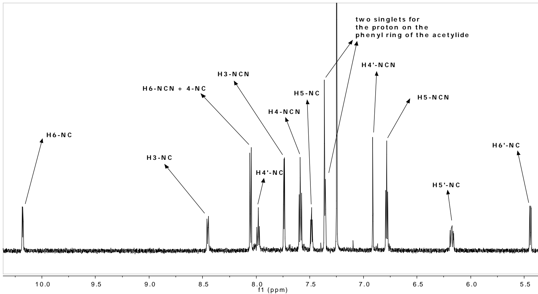
Figure 2.60: ^1\text{H-NMR} spectrum of \text{Ir}(\text{L1})(\text{dFppy})(\text{A1}) (30).
