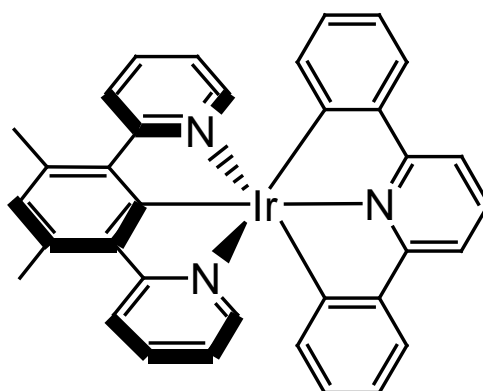
Figure 1.22 (87) : example of \text{Ir}(\text{N}^{\wedge}\text{C}^{\wedge}\text{N})(\text{C}^{\wedge}\text{N}^{\wedge}\text{C}) complex
