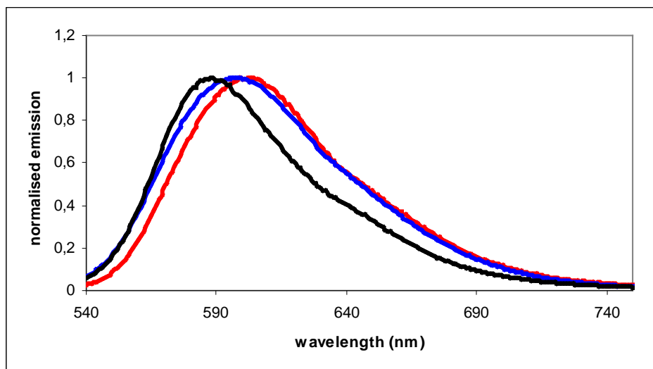
Figure 3.29: emission spectra in dichloromethane at room temperature of the complexes, Ir(L3)(ppy)(A5) ( 35 ) (blue line), Ir(L3)(ppy)(A1) ( 31 ) (red line), Ir(L3)(ppy)Cl ( 5 ) (black line).
