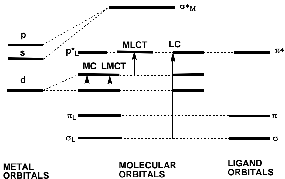
Figure 1.2: Schematic energy-level diagram for an octahedral transition metal complex. The various kinds of electronic transitions are also indicated.
