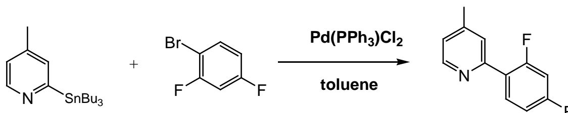
Figure 2.22: scheme for the synthesis of 1,3-di-fluoro-phenyl-4-methoxypyridine.
