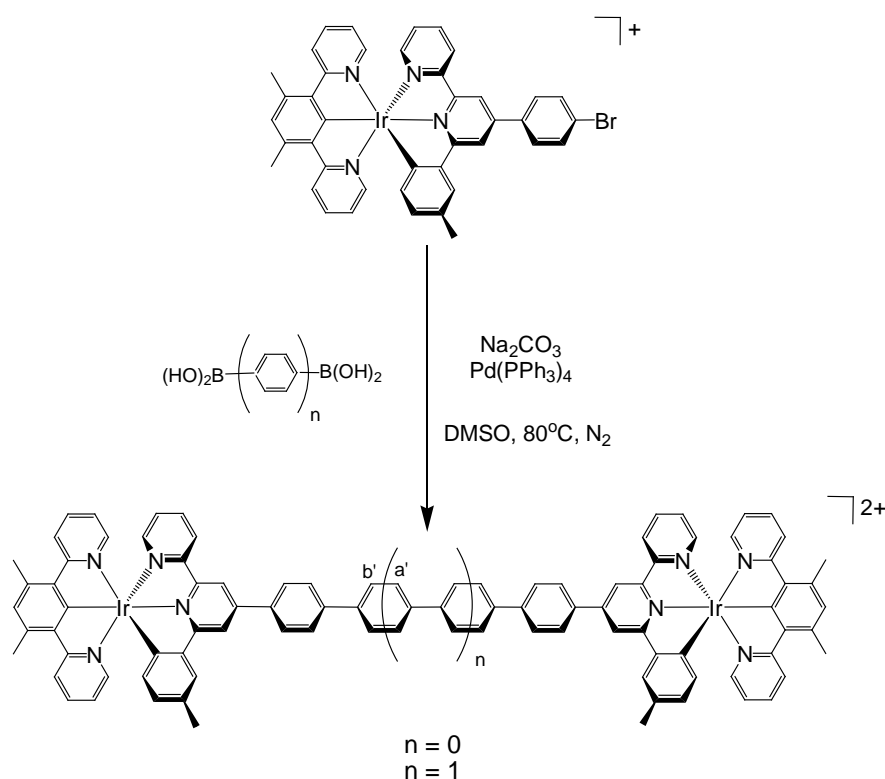
Figure 4.7 (24) : scheme for the synthesis of homo-metallic dinuclear complexes previously reported by our research group
