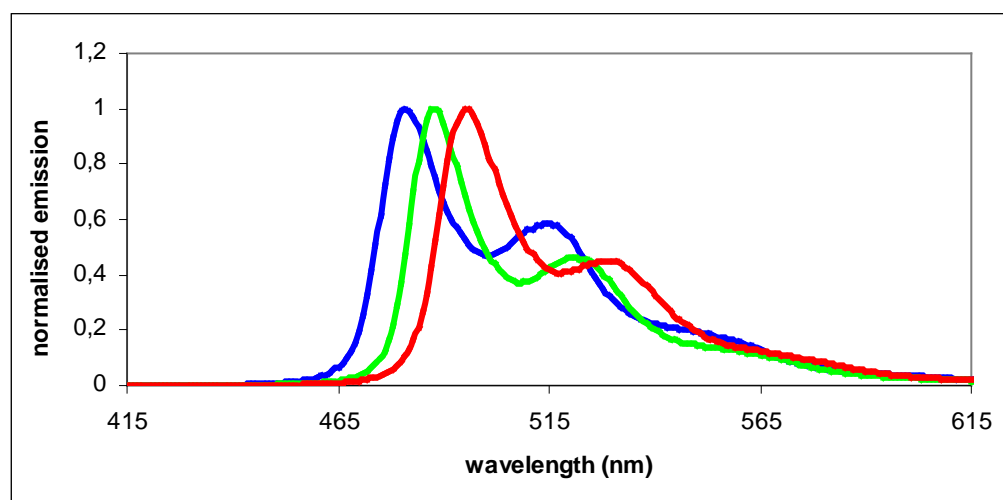
Figure 3.26: emission spectra in dichloromethane at room temperature of the complexes Ir(L1)(dFppy)CN ( 22 ) (blue line), Ir(L1)(dFppy)SCN ( 27 ) (green line), Ir(L1)(dFppy)Cl ( 1 ) (red line).
