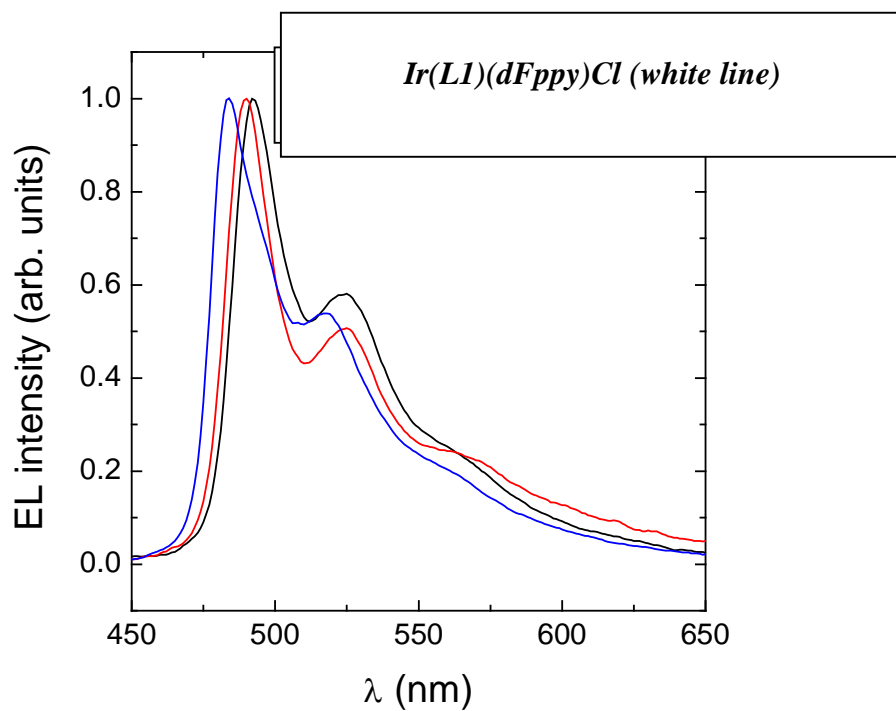
Figure 3.28: EL spectra and CIE diagram for the complexes Ir(L1)(dFppy)CN ( 22 ) and Ir(L1)(dFppy)SCN ( 27 ) compared to that of Ir(L1)(dFppy)Cl ( 1 ).
