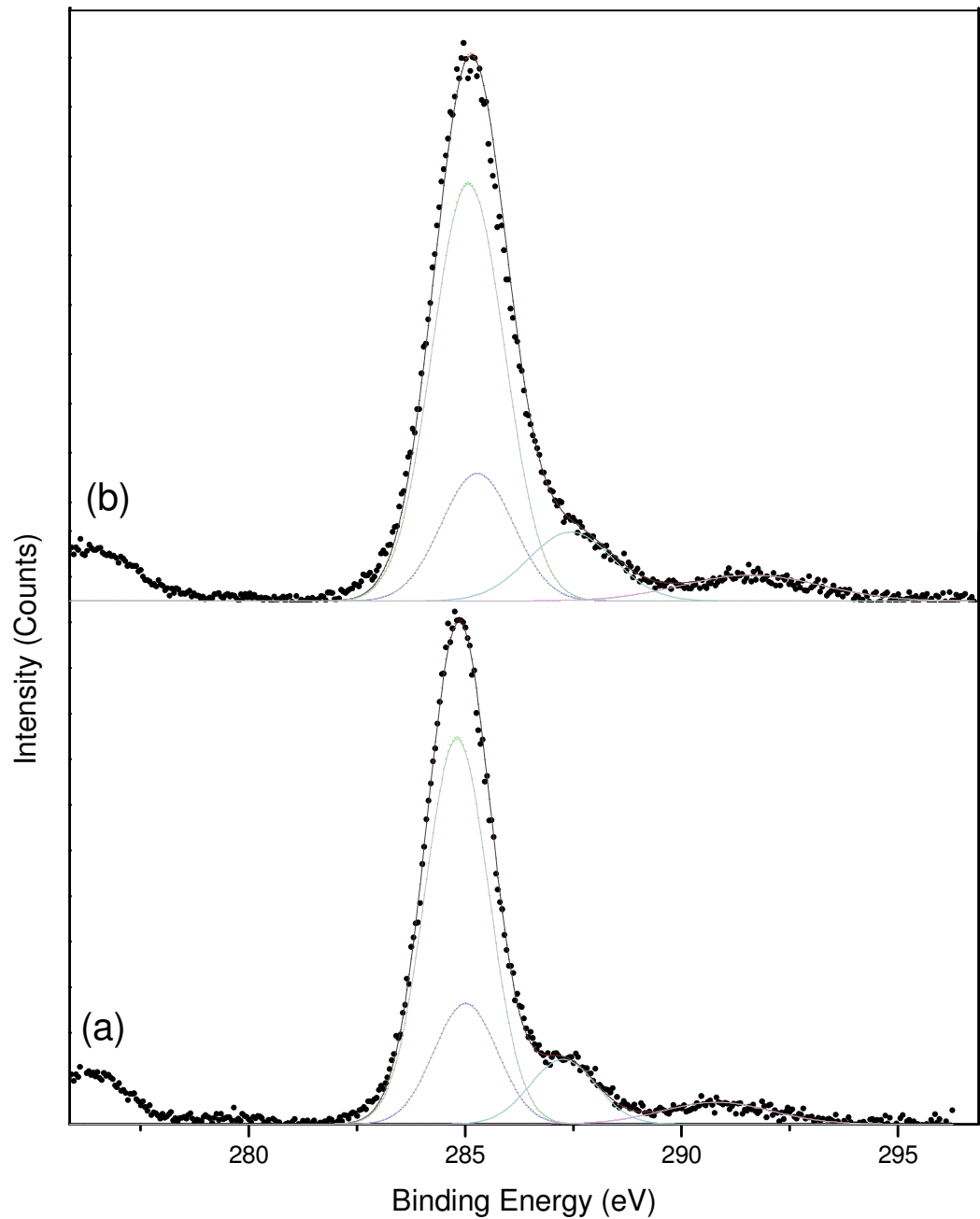
Figure 4.1. 3-Vinylbenzaldehyde Plasma Polymer Carbon XPS Envelopes. (a) 50µs-on, 4ms-off Pulsed Plasma Polymer. (b) 5W Continuous Wave Plasma Polymer.
