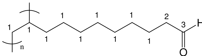
Figure 3.3. Theoretical surface polymer structure indicating the three expected carbon environments 1) \underline{C}_yH_x 2) \underline{C}-C=O 3) \underline{C}=O
