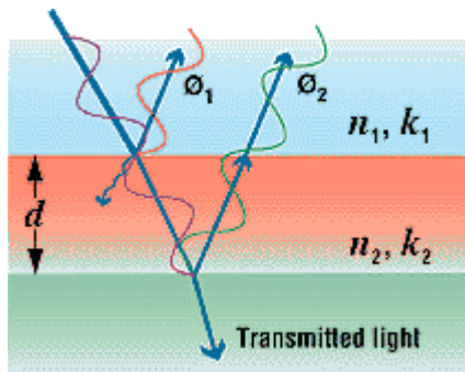
Figure 2.8. Reflections from a thin film on a substrate.
