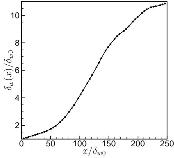
Figure 5.36: Vorticity thickness growth in the mixing layer
