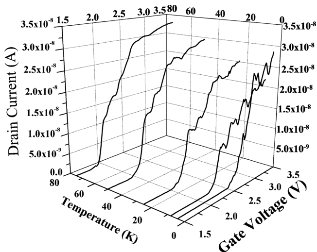
FIG. 2. Measured drain current in a junctionless n-channel transistor as a function of gate voltage and temperature. Drain voltage is 100 mV.
