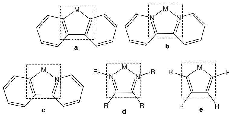
Figure 1.27: Examples of metallacyclopentadiene complexes.
