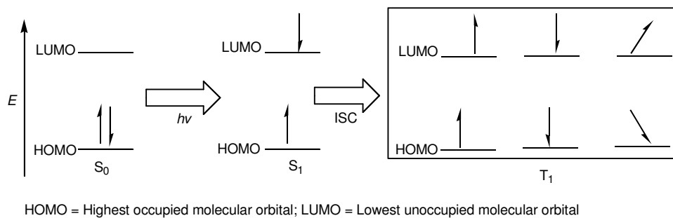
Figure 1.2: General diagram of the electron orientation in the ground ( S_0 ), singlet ( S_1 ) and triplet ( T_1 ) excited states of a molecule for HOMO-LUMO transition.
