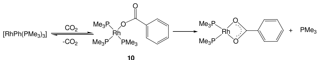
Figure 3.46: Synthesis of [\text{Rh}(\eta^2\text{-O}_2\text{CPh})(\text{PMe}_3)_2] by Darensbourg and co-workers. 33
