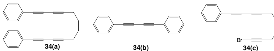
Figure 2.33: Three products obtained from Cadiot-Chodkiewicz coupling.
