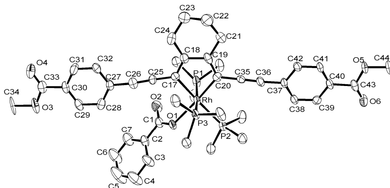
Figure 3.53: Molecular structure of 11(c) . Hydrogen atoms and the C 6 H 14 molecule are omitted for clarity (thermal ellipsoids are shown at 50% probability).
