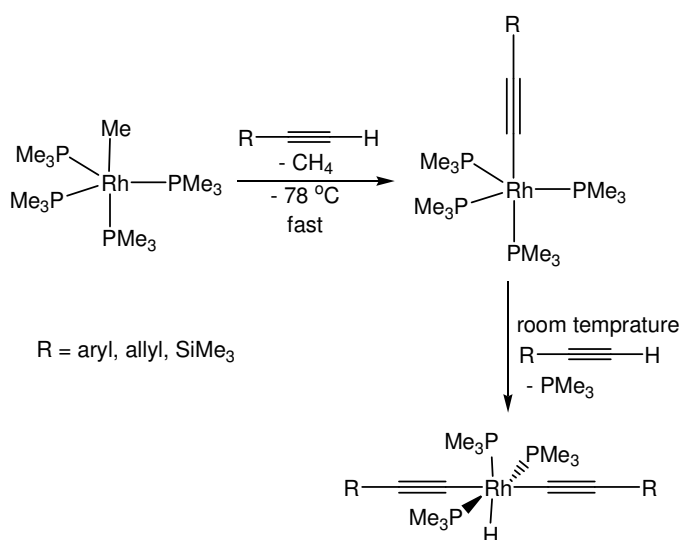
Figure 3.14: Formation of mer,trans - [\text{RhH}(-\text{C}\equiv\text{C-R})_2(\text{PMe}_3)_3] by adding excess
