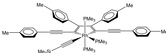
Figure 3.1: The structure of 2,5-bis( p -tolylethynyl)-3,4-bis( p -tolyl)rhodacyclopentadiene.
