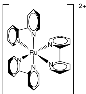
Figure 1.17: Structure of [Ru(bpy) 3 ] 2+ .
