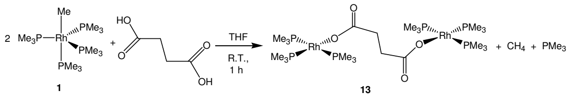
Figure 3.47: Synthesis of the di-rhodium complex 13 using succinic acid.
