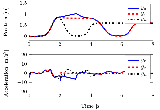
Fig. 7. Similar to Fig. 6, except that y_a was moved away from the nominal path between 2s to 3s. Again, the behavior was satisfactory both regarding position and acceleration.
