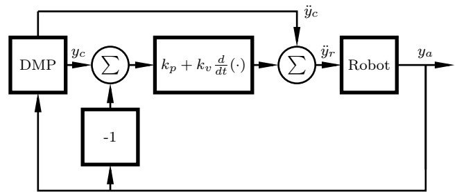
Fig. 4. Schematic overview of the control structure described in Sec. 4. The block denoted 'Robot' includes the internal controller of the robot.
