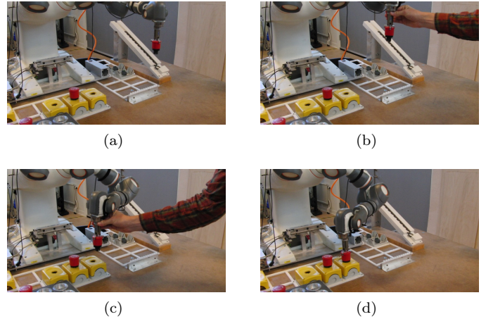
Fig. 10. First scenario. In (a), the robot started to execute a DMP for placing the stop button in the rightmost yellow case. A human perturbed the motion twice. The first perturbation (b) was formed by moving the end-effector away from its path, and then releasing it. The second perturbation (c) lasted for a longer time, and consisted of unstructured movement. The robot recovered from both perturbations, and managed to place the stop button in the case (d). Data from one trial are shown in Fig. 12.
