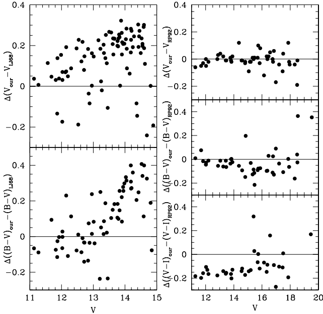
Figure 2. Magnitude and colour differences between our values and those by LJ68 for 111 stars in common (left-hand panels) and our values and those by RP92 for 60 stars in common (right-hand panels) as a function of V .
