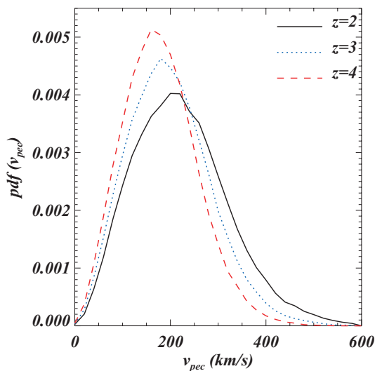
Figure 3. Probability distribution functions (PDFs) of the peculiar velocity of the absorbing gas along 1000 random LOS through our simulation box at three different redshifts as indicated. Note that we are not using the value of the velocity’s component along the LOS, but rather the modulus of the full three-dimensional velocity.
