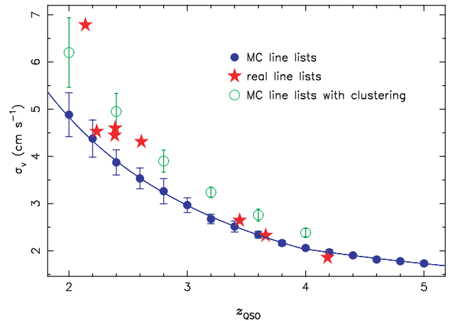
Figure 8. Comparison of \sigma_v measurements derived from simulated MC line lists (blue dots and solid line, same as in Fig. 7) and from real line lists (red stars). The green circles show the results derived from simulated MC line lists that include a simple scheme for clustering absorption lines in redshift space (see text for details).
