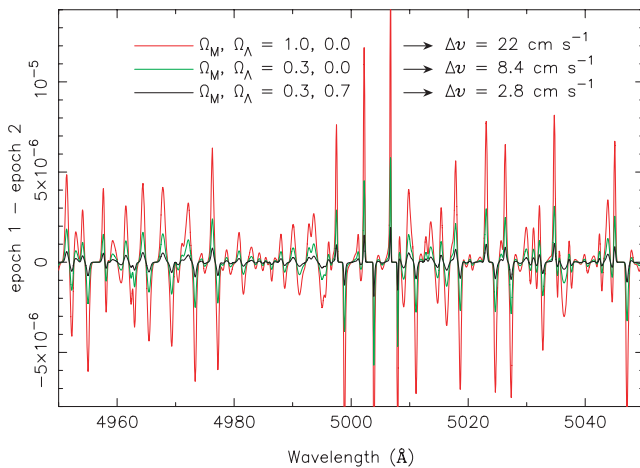
Figure 6. Flux difference between two artificial, noiseless spectra of the same Ly \alpha forest at z \approx 3 simulated for two observing epochs separated by \Delta t_0 = 10 yr and for various combinations of \Omega_M and \Omega_\Lambda as indicated. The redshift drift implied by these parameters is also given.
