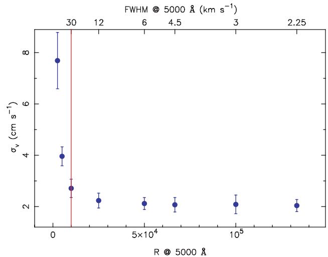
Figure 9. Radial velocity accuracy as a function of spectral resolution. Each point and error bar is the mean and \pm 1 rms of 10 simulations at z_{\text{QSO}} = 4 and S/N = 13 000. The pixel size is kept constant and is chosen such that a resolution element is sampled by 3 pixels at the highest resolution considered. The labels along the bottom axis denote the resolving power at 5000 \text{\AA} , while the labels along the top axis show the equivalent FWHM of an unresolved line. The vertical red line marks the mode of the absorption lines’ b parameter distribution (cf. equation 7).
