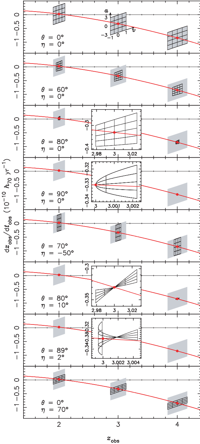
Figure A2. Top panel: the solid line shows the cosmological redshift drift, \dot{z}(z) , expected for comoving sources (cf. Fig. 2). The three grids show how an object at z = 2, 3 and 4 , respectively, moves in the observed z_{\text{obs}} - \dot{z}_{\text{obs}} plane as a function of v and a , assuming \theta = \eta = \zeta = 0 . For each grid, the vertical lines are lines of constant v , while the tilted horizontal lines are lines of constant a . The values of v and a are indicated along the middle grid in units of 10^4 \text{ km s}^{-1} and 10^{-8} \text{ cm s}^{-2} . The other panels show the same for different values of \theta and \eta as indicated (and \zeta = 0 ). For comparison, the grey shaded areas in each panel are the same as in the top panel. The insets show a blow-up of the region around the z = 3 point.
