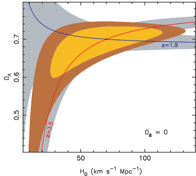
Figure 16. Expected constraints in the \Omega_\Lambda – H_0 plane for flat cosmologies assuming O = 2 and \Delta t_0 = 20 yr and using the same two redshift drift measurements as in Fig. 15. The red and blue solid lines and the grey shaded bands show the individual constraints provided by each of the two objects. The coloured ellipses show the joint 68 and 90 per cent confidence regions that result from combining the two measurements.
