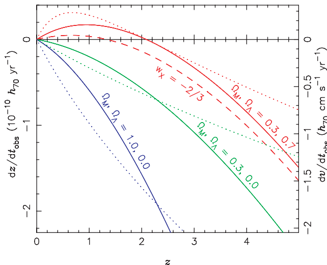
Figure 2. The solid (dotted) lines and left-hand axis (right-hand axis) show the redshift drift \dot{z} ( \dot{v} ) as a function of redshift for various combinations of \Omega_M and \Omega_\Lambda as indicated. The dashed line shows \dot{z} for the case of dark energy having a constant w_X = -2/3 (and \Omega_M, \Omega_X = 0.3, 0.7 ).
