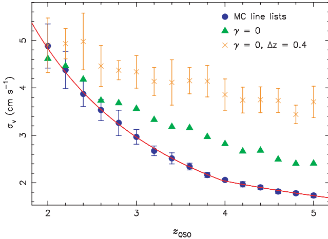
Figure 7. The blue dots with error bars show the accuracy with which a radial velocity shift can be determined from a Ly \alpha forest spectrum as a function of QSO redshift. The red line parametrizes the redshift dependence as in equation (14). Each point is the mean \sigma_v measured from 10 pairs of artificial spectra with S/N = 13 000, generated from simulated MC absorption line lists. The error bars show the \pm 1 rms range of the 10 simulations. The green triangles show the results for simulations where the redshift evolution of the Ly \alpha forest has been switched off, i.e. where \gamma = 0 (cf. equation 7). The orange crosses show the result of also restricting the \sigma_v measurement in each spectrum to a redshift path of constant length \Delta z = 0.4 , as opposed to using the full Ly \alpha forest region between the QSO's Ly \alpha and Ly \beta emission lines.
