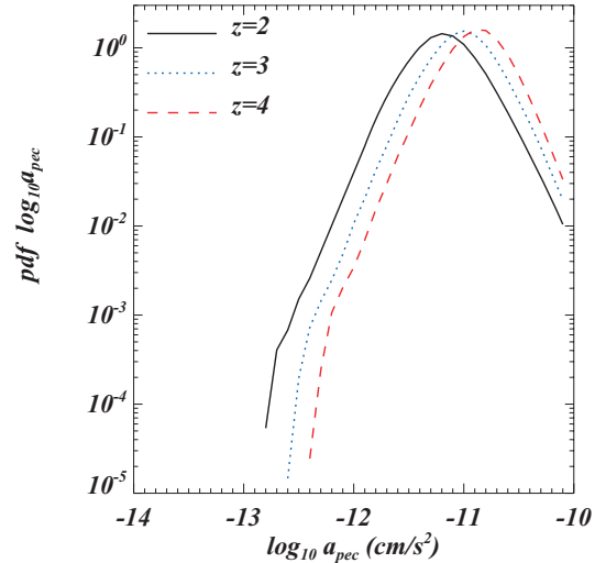
Figure 4. As Fig. 3 for the peculiar acceleration.
