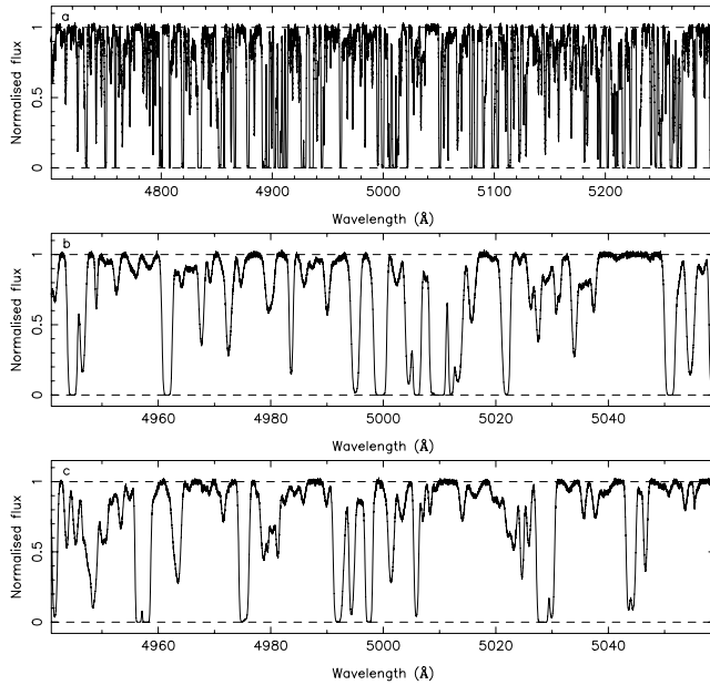
Figure 5. (a) Example of an artificial Ly \alpha forest spectrum at z \approx 3 generated from an MC absorption line list. (b) Close-up of the region around 5000 Å. (c) Artificial spectrum generated from the observed line list of Q0302–003. Both spectra have S/N = 100.
