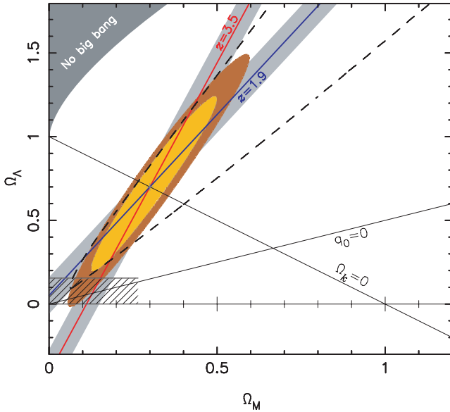
Figure 15. Expected constraints in the \Omega_\Lambda - \Omega_M plane from two measurements of the redshift drift at two different redshifts as indicated, assuming O = 2 and \Delta t_0 = 20 yr. The two targets and the split of the observing time among them were chosen to give the best lower limit on \Omega_\Lambda . The red and blue solid lines and the grey shaded bands show the individual constraints provided by each of the two objects assuming a fixed h_{70} = 1 . The coloured ellipses show the joint 68 and 90 per cent confidence regions that result from combining the two measurements, marginalizing over H_0 using an external prior of H_0 = (70 \pm 8) \text{ km s}^{-1} \text{ Mpc}^{-1} . The hashed region indicates the 95 per cent lower limit on \Omega_\Lambda . The dashed contour shows the 68 per cent confidence region that results from using a flat prior on H_0 and just marginalizing over the range 0 \leq H_0 \leq 140 \text{ km s}^{-1} \text{ Mpc}^{-1} . Flat cosmologies and the boundary between current deceleration and acceleration are marked by solid black lines. The dark shaded region in the upper left-hand corner designates the regime of ‘bouncing universe’ cosmologies which have no big bang in the past.
