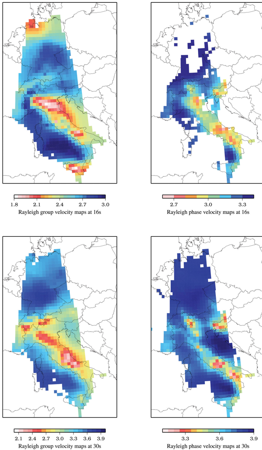
Figure 10. Group- (left-hand panel) and phase- (right-hand panel) velocity maps at 16 s (top panel) and 30 s (bottom panel) in km s -1 .
