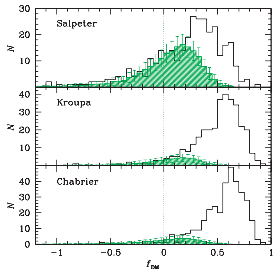
Figure A1. Distributions of DM fraction for ETGs. The open histograms are the observational results, with a different IMF for each panel (as labelled). The shaded green histograms are random realizations of galaxy subsamples having intrinsic f_{\text{DM}} = 0.1 , with error bars illustrating the approximate Poissonian uncertainties. See the text for further details.
