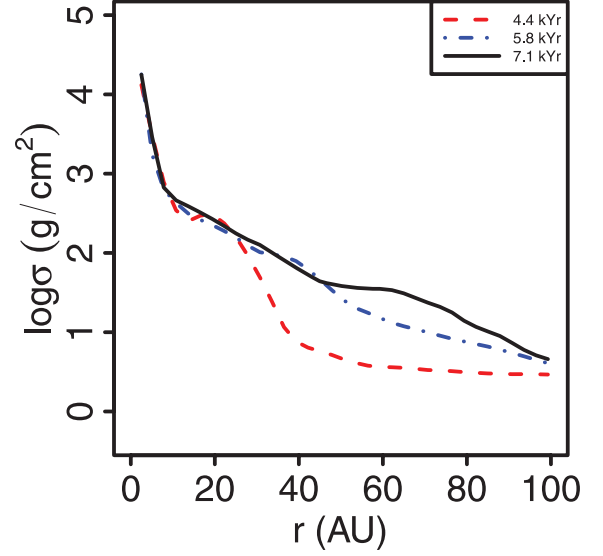
Figure 7. Evolution of the surface density profile of the isolated system. \sigma tends to increase at all radii with time.
