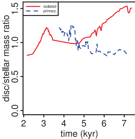
Figure 6. The ratio of disc mass to accreted stellar mass versus time, for the isolated and primary systems.
