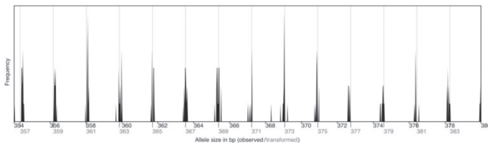
Fig. 1. Frequency histogram for one marker from data set 1. Black labels refer to observed allele sizes, while transformed allele sizes are shown with grey labels (in bp). Observed alleles do not conform to dinucleotide periodicity, but transformed alleles match the expected pattern.
