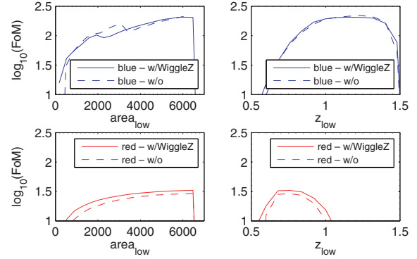
Figure 8. The FoM as a function of area (left-hand panels) and redshift (right-hand panels) for a single-bin survey at low redshift using either line emission (top) or continuum emission (bottom) galaxies, with (solid curves) and without (dashed curves) the WiggleZ measurement at z = 0.75 .
