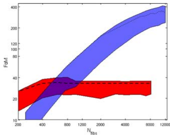
Figure 6. The variation of the FoM of the optimal survey with the total number of spectroscopic fibres, for both line-emission galaxies (dotted curve) and continuum galaxies (dashed curve), for a single bin at low redshift. The line-emission curve does not reach an asymptotic limit before 10 000 fibres, whereas the continuum curve reaches its asymptotic value at around 750 fibres. We also include the effect of varying the number counts models of the galaxies in a band between ‘pessimistic’ and ‘optimistic’ limits (line-emission in blue and continuum-emission in red). This extra freedom does not change the results concerning number of fibres. For a small number of fibres, the optimistic and default models give the same FoM, as the optimal surveys have reached the maximum number of pointings and smallest exposure time, and no more galaxies can be observed. We assume that fibres can access any part of the FoV.
