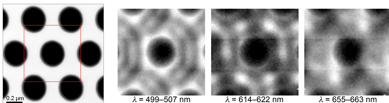
FIG. 2. STEM image (left) of PhC tile structure with region chosen for CL spectrum image (SI) marked by the square. SI data was acquired for 75 x 75 pixels with a 500–775 nm wavelength range with an acquire time of 15 s per pixel for a total map time of 23 h. On the right are three slices of the SI CL data cube, after filtering to remove cosmic X-ray spikes and binning the wavelength axis by 40 times. Strong CL wavelength-dependent spatial modulations are seen. Horizontal lines probably result from detector gain variations resulting from temporary CCD temperature fluctuations.
