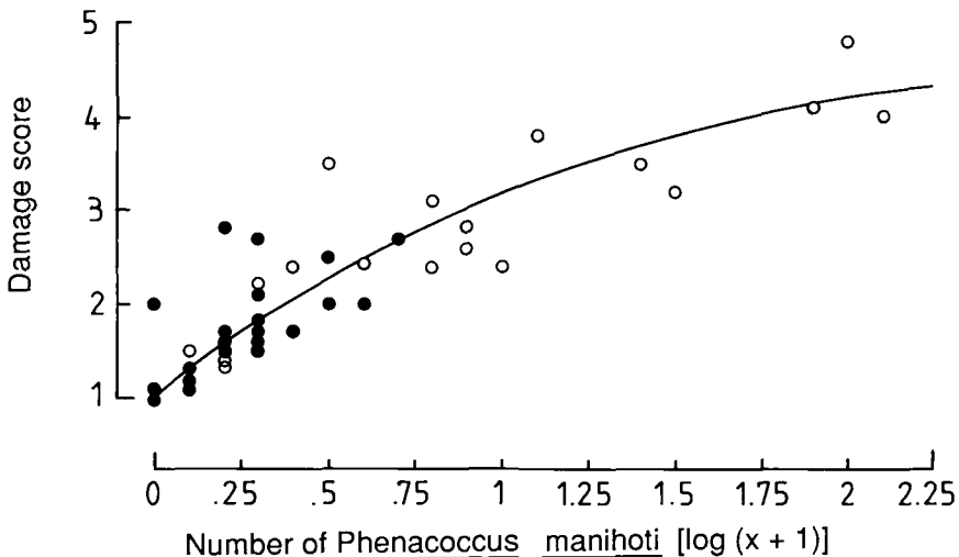
Fig. 2.—Damage score of cassava shoot tips (parameter 24, Appendix and text) as a function of present Phenacoccus manihoti density in 60 fields in Ghana and Ivory Coast in February–March 1986. (O), Fields in areas where Epidinocarsis lopezi was lacking or had been introduced only recently; (●), fields in areas where E. lopezi had been present since the first half of the cropping season.
