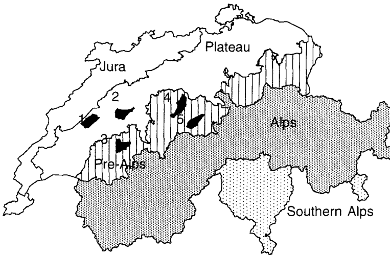
FIG. 1. The five areas of study on the Swiss Plateau and the Pre-Alps. 1: Payerne; 2: Bern West; 3: Schwarzsee; 4: Entlebuch; 5: Glaubenberg.
