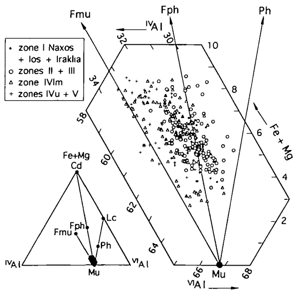
Fig. 10. ^{IV}Al - ^{VI}Al -(Fe + Mg) diagram for metabauxitic muscovite (atomic proportions). Muscovite-phengite (Mu-Ph), muscovite-ferriphengite (Mu-Fph) and muscovite-ferrimuscovite (Mu-Fmu) exchange vectors are indicated in the diagram. Cd, celadonite, K_2(Fe^{2+}, Mg)_2Fe^{3+}(Si_8O_{20})(OH)_4 ; Fmu, K_2Fe^{3+}Al_2(Al_2Si_6O_{20})(OH)_4 ; Fph, K_2(Fe^{2+}, Mg)Fe^{3+}Al_2(AlSi_7O_{20})(OH)_4 ; Lc, leucophyllite, K_2(Fe^{2+}, Mg)_2Al_2(Si_8O_{20})(OH)_4 ; Mu, K_2Al_4(Al_2Si_6O_{20})(OH)_4 ; Ph, K_2(Fe^{2+}, Mg)Al_3(AlSi_7O_{20})(OH)_4 .
