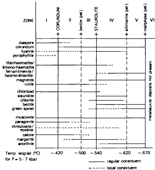
Fig. 3. Mineralogy of the metabauxites throughout the metamorphic zones of Naxos (Feenstra, 1985). The diagram only depicts primary mineral occurrences. Metamorphic zones and isograds are shown in Fig. 2.
