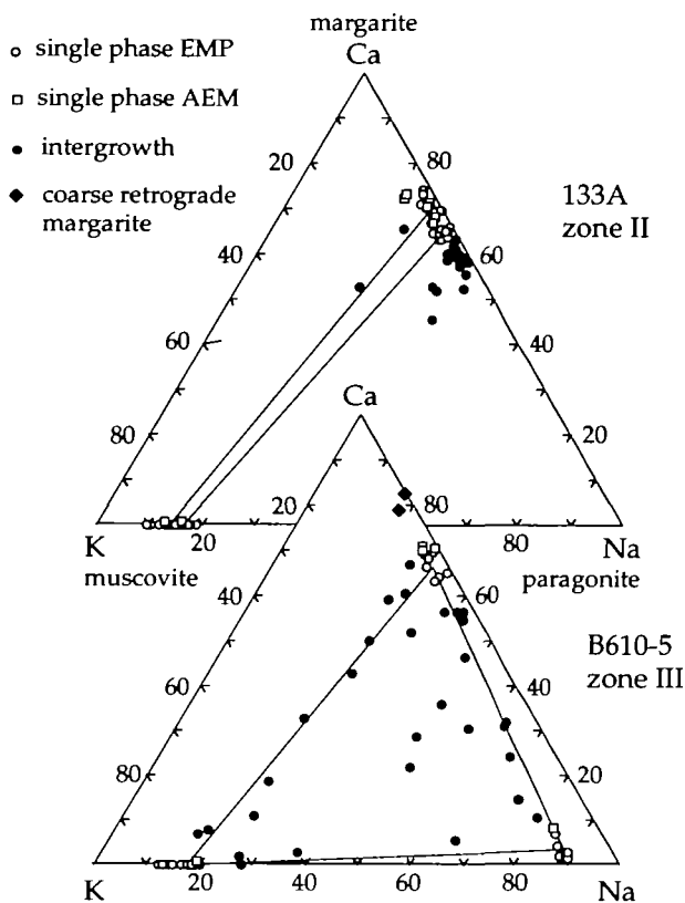
Fig. 6. Ca-Na-K diagram (atom %) depicting EMP and AEM analyses of white micas in samples 133A and B610-5. Tie-lines connect average compositions of micas in close contact. Margarite in sample 133A is locally interleaved with thin (<500 Å thick) paragonite lamellae which are too small for successful AEM analysis (see Fig. 5a and b).
