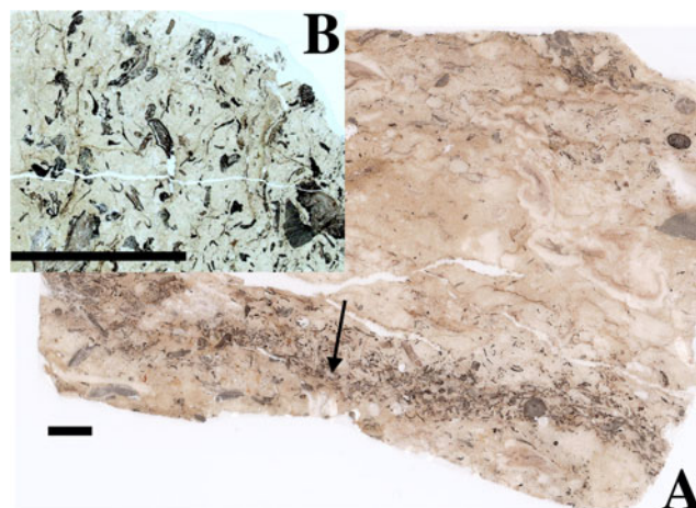
Figure 1. A: Photograph using top illumination of cellulose acetate peel of limestone block containing charcoalfied plants (arrow shows charcoalfied plant layer) from the late Viséan (mid-Mississippian, Carboniferous) of Kingswood, Scotland (KIN 1019B); scale bar = 1 cm. B: Transmitted light micrograph of polished rock thin section of Block KIN 957I showing charcoalfied plants; scale bar = 1 cm.
