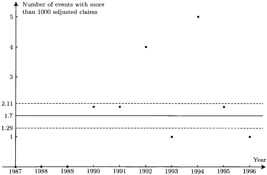
FIGURE 4.1: Observed number of events in the ten observation periods November 1st to October 31st causing more than 1000 adjusted claims. The empirical mean of \lambda_{1000}^{\text{const}} = 1.7 events per observation period is also shown. The dashed lines indicate the estimated standard deviation 0.41 of the estimator \lambda_{1000}^{\text{const}} given by (4.4). The estimated standard deviation for the distribution of the observations is (\lambda_{1000}^{\text{const}})^{1/2} = \sqrt{1.7} \approx 1.30 .
