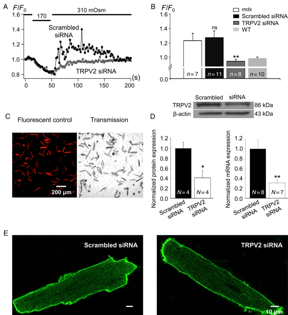
Figure 5 siRNA ablation of TRPV2 in mdx cardiomyocytes. (A) Time courses of normalized Ca^{2+} -related fluorescence pooled from mdx myocytes transfected with siRNA directed against TRPV2 (grey circles) or scrambled siRNA as a negative control (black circles). Line on the top represents the protocol by which extracellular solutions were changed. (B) Mean values of normalized fluorescence during 40 s after the osmotic shock obtained from untransfected mdx myocytes, mdx cells transfected with scrambled siRNA, mdx cells transfected with siRNA against TRPV2 and WT cardiomyocytes. WT data replotted for comparison. (C) Fluorescence and transmission images of mdx ventricular cardiomyocytes showing successful transfection with fluorescently labelled siRNA. (D) Statistical analysis of reduced protein and mRNA expressions by western blot (left and inset) and by RT-PCR (right) in mdx cardiomyocytes after transfection with siRNA directed against TRPV2. (E) Confocal images of T-tubular network with di-8-ANEPPS membrane staining after transfection with scrambled siRNA and siRNA against TRPV2, respectively. n = 7-11 , N = 4-8 . * P < 0.05 , ** P < 0.01 , ns, not significant.
