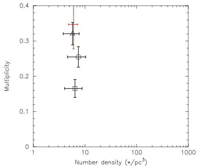
Figure 21. Multiplicity versus stellar density in the separation range 18–830 au for the simulated Taurus-like clusters (see Table 4 for details). The observed value in Taurus is shown by the red data point.
